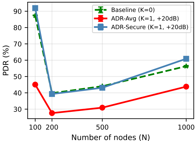
PDR Scalability: Baseline vs Attack vs Defense
