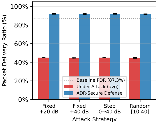
PDR Under Fixed vs Adaptive Byzantine Attacks (3 GWs, N=100 nodes, K=1 Byzantine GW)
