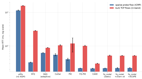
Sparse probe vs bulk flow latency — staged workload fq_codel's new-flow heuristic privileges the probe, so the two differ; quoting only the probe overstates the benefit for bulk traffic
