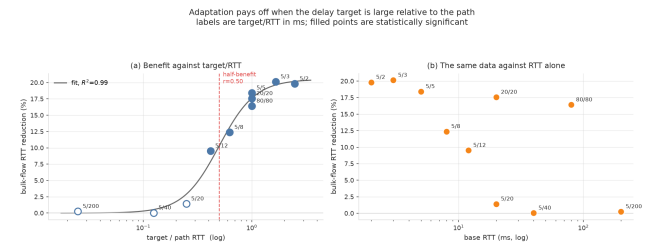
Figure 4: The central result. Left: adaptation benefit against r = \text{target}/\text{RTT} , collapsing onto a single saturating curve. Right: the same measurements against path RTT alone, where they do not collapse. Filled points are statistically significant; labels give target/RTT in ms.
