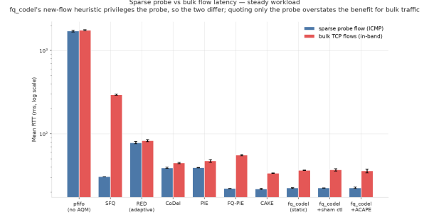
Figure 8: Sparse probe flow against bulk TCP flow round-trip time, measured separately. Flow-queueing disciplines privilege sparse flows by construction, so a single latency number averages two populations the mechanism treats differently. The ratio between them ranges from 1.1 to 9.6 across the systems tested, which is why both are reported throughout rather than one.
