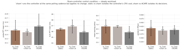
Figure 6: The sham-controller condition. The sham polls at the same cadence as the real controller and applies no parameter change, so any difference between sham and static is the controller's computational cost rather than the effect of its decisions. Without this condition the two are confounded.
