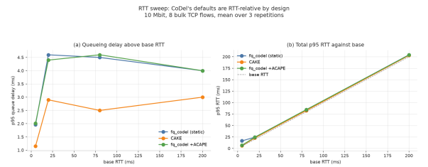
Figure 9: The RTT sweep that motivated the scaling law. Adaptation recovers a large and highly significant share of bulk-flow RTT on a short path and nothing at 20, 80 or 200 ms. Read as four separate measurements this is unexplained; read through r = \text{target}/\text{RTT} it is one curve, which is the argument of Figure 4.
