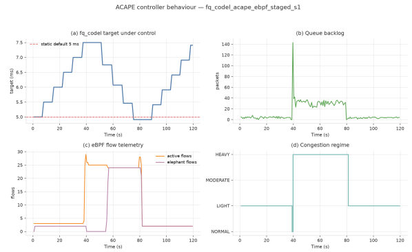
Figure 3: The controller acting: regime classification, the parameter trajectory it produces, and the queue it is responding to. A controller that classifies but never adjusts is indistinguishable from the static configuration in a summary statistic, so the adjustment count is reported for every cell.
