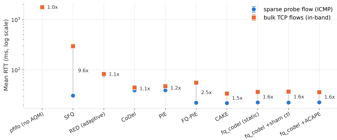
Figure 11: fig02_latency_sparse_vs_bulk_steady.png. Sparse probe flow vs bulk TCP flow RTT, why the two differ (steady workload)
