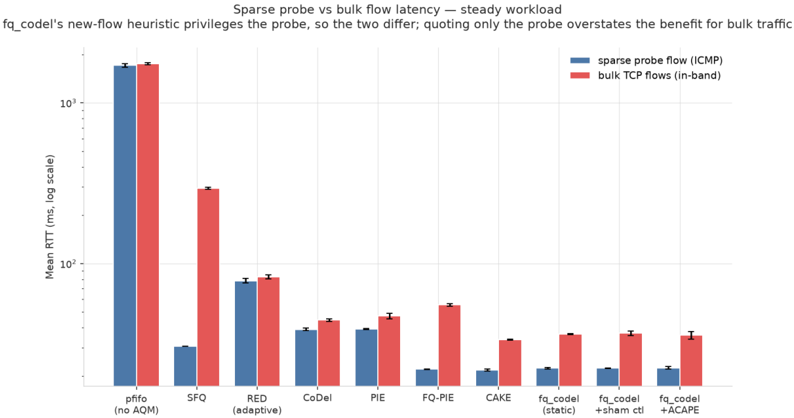
Figure 11: fig02_latency_sparse_vs_bulk_steady.png. Sparse probe flow vs bulk TCP flow RTT, why the two differ (steady workload)
