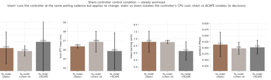
Figure 6: The sham-controller condition. The sham polls at the same cadence as the real controller and applies no parameter change, so any difference between sham and static is the controller's computational cost rather than the effect of its decisions. Without this condition the two are confounded.
