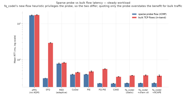
Figure 8: Sparse probe flow against bulk TCP flow round-trip time, measured separately. Flow-queueing disciplines privilege sparse flows by construction, so a single latency number averages two populations the mechanism treats differently. The ratio between them ranges from 1.1 to 9.6 across the systems tested, which is why both are reported throughout rather than one.
