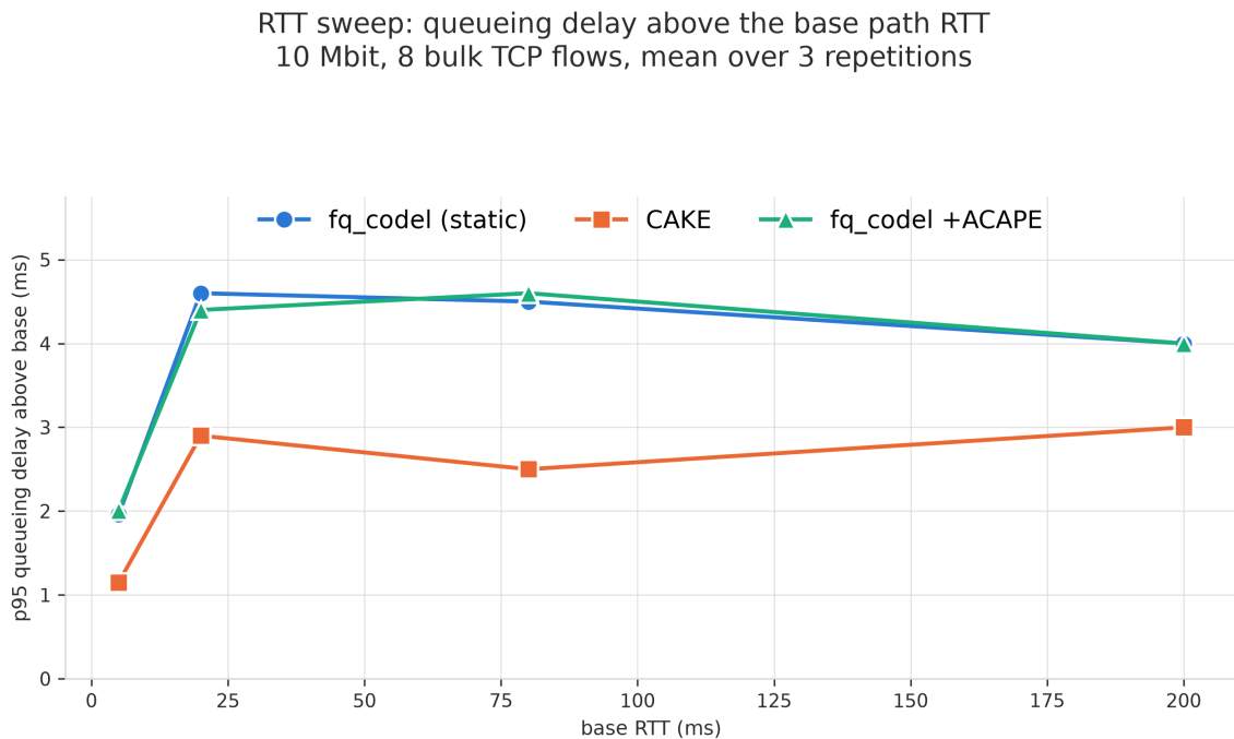
Figure 16: fig15_rtt_sweep.png, fig15_rtt_sweep
