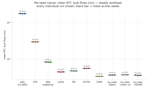
Figure 10: Every individual run shown rather than only its summary. Each point is one repetition of one configuration, with the mean marked. Run-to-run spread is the quantity the confidence intervals describe, and showing it makes visible both the cases where three repetitions agree closely and the cases where they do not.
