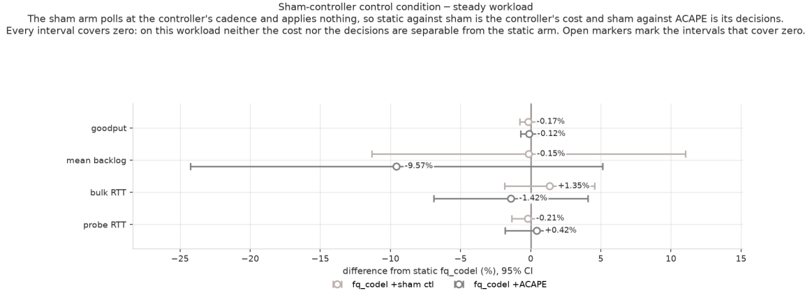
Figure 14: fig13_sham_control_steady.png. Sham-controller condition, separates controller CPU cost from control decisions (steady workload)
