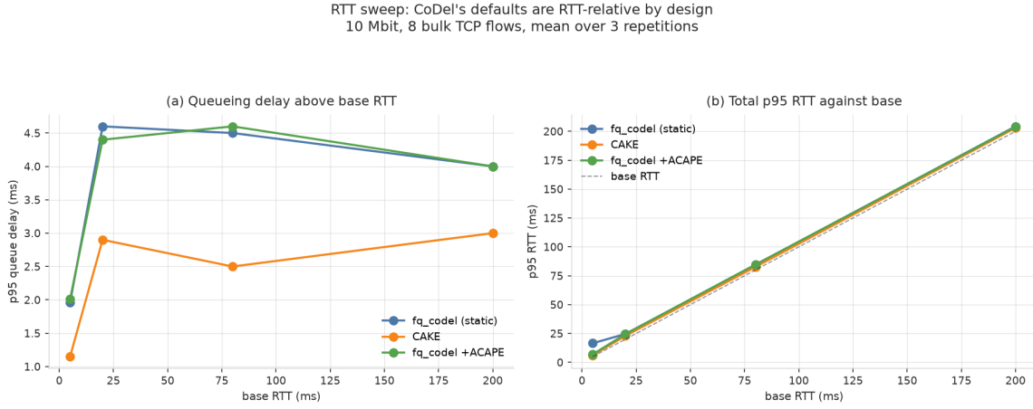
Figure 22: fig15_rtt_sweep.png, fig15_rtt_sweep
