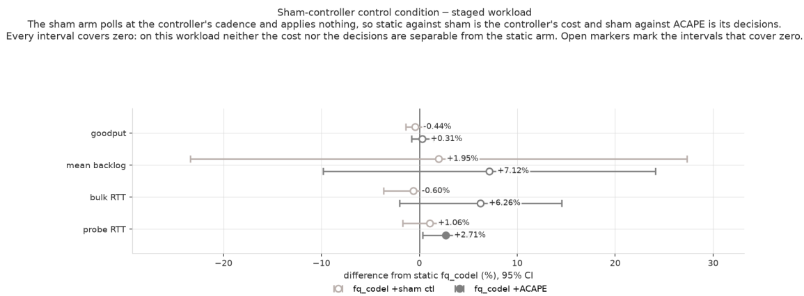
Figure 46: fig13_sham_control_staged.png. Sham-controller condition, separates controller CPU cost from control decisions (staged workload)
