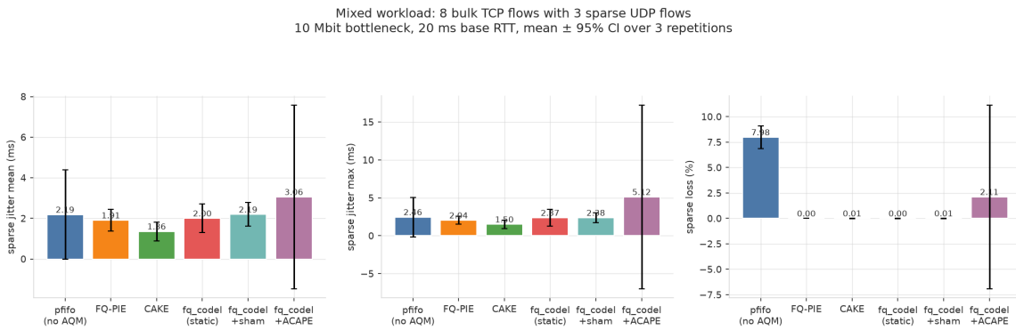
Figure 21: fig14_mixed_workload.png, fig14_mixed_workload
