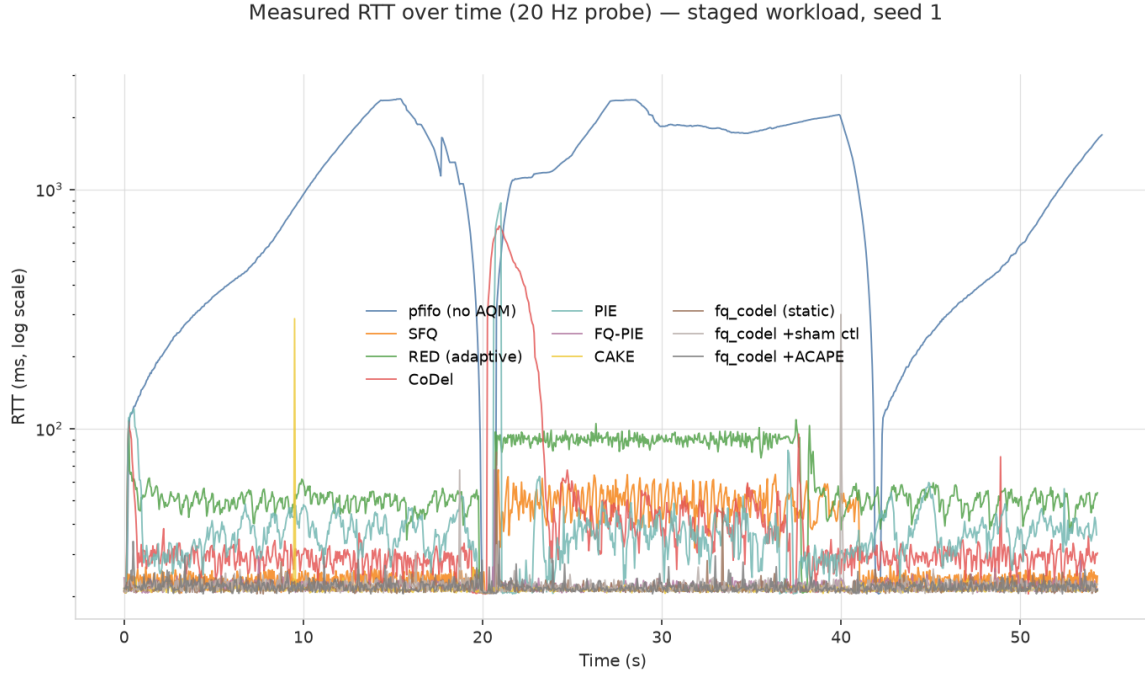
Figure 20: fig11_timeseries_rtt_staged.png. Measured RTT over time (20 Hz probe) (staged workload)
