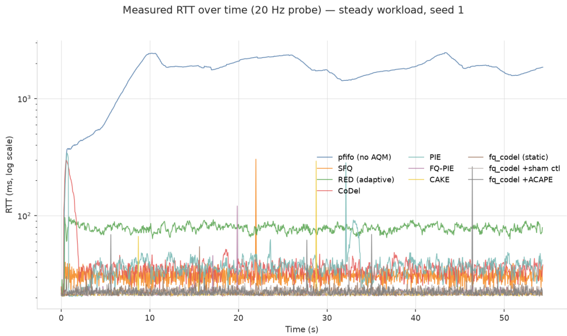
Figure 45: fig11_timeseries_rtt_steady.png. Measured RTT over time (20 Hz probe) (steady workload)
