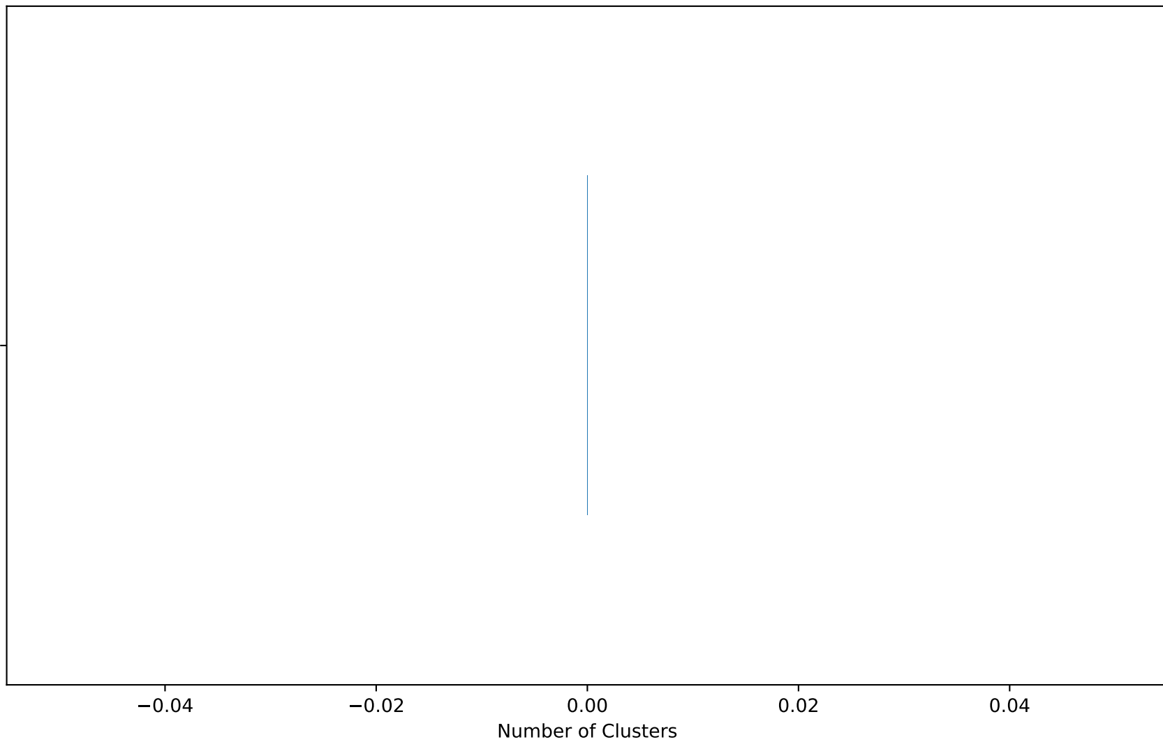
Number of Found Clusters for Target: Ipa5104
