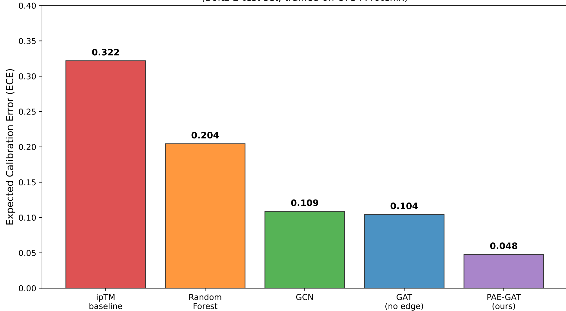
Ablation Study — PAE-GAT Components (Boltz-2 test set, trained on OF3+Protenix)
