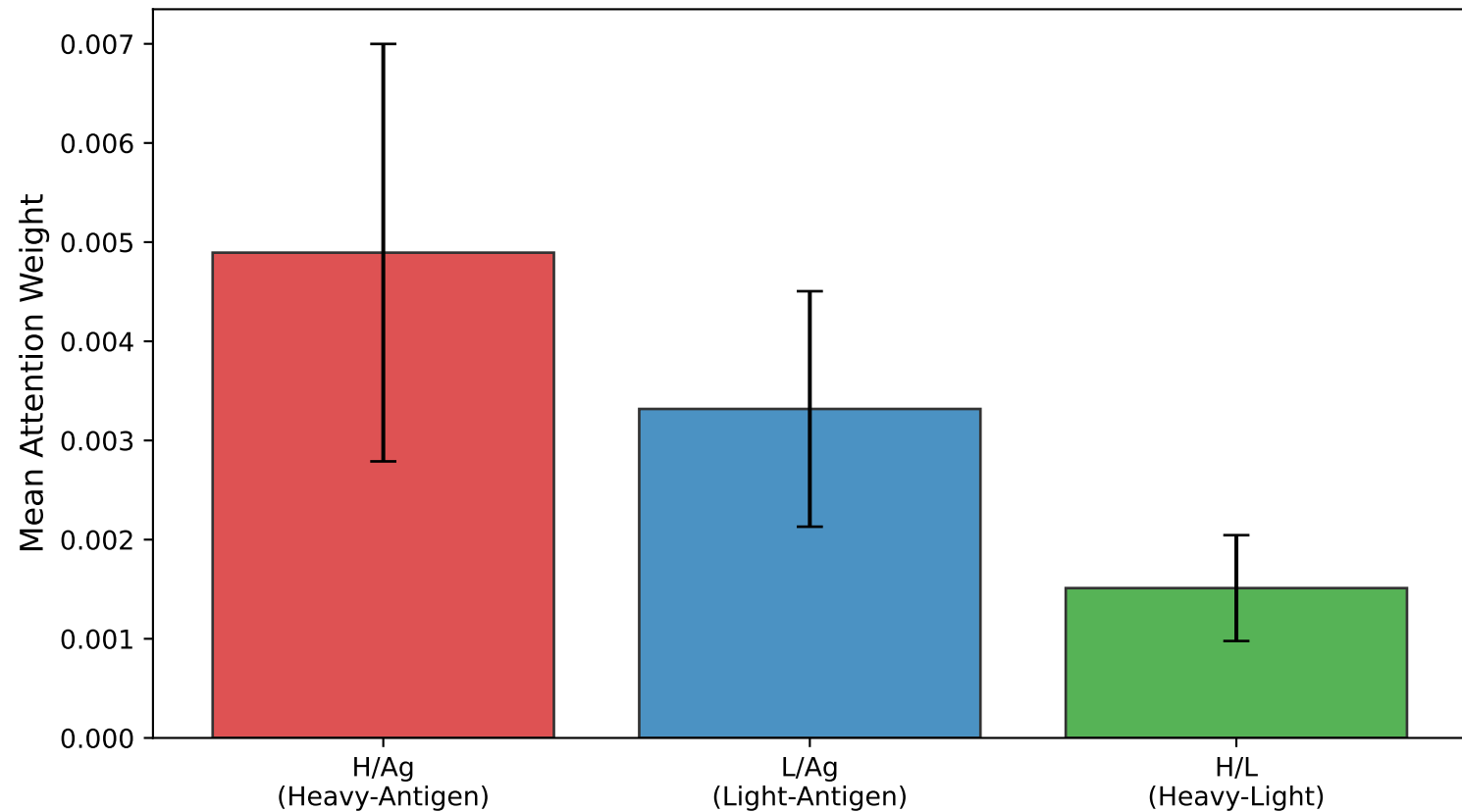
PAE-GAT Learned Attention by Interface Type (Round 1 model, Boltz-2 test set)
