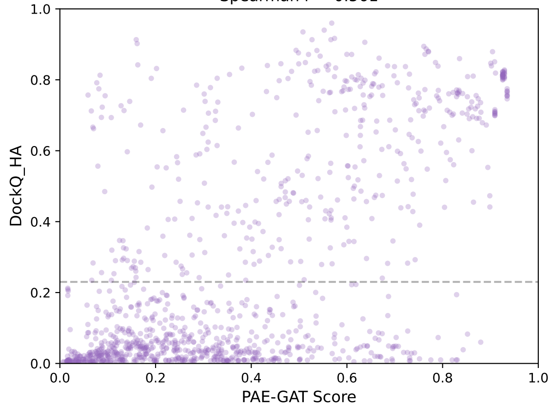
PAE-GAT vs DockQ_HA (Boltz-2) Spearman r = 0.561
