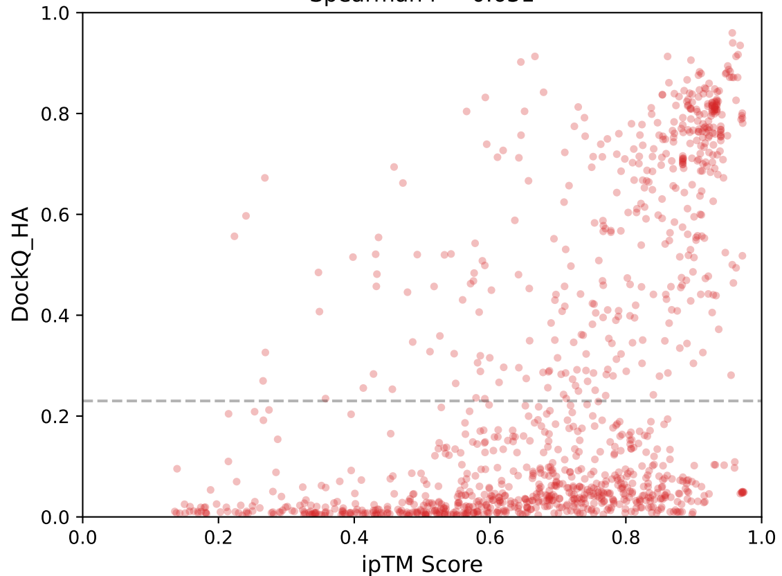
ipTM vs DockQ_HA (Boltz-2) Spearman r = 0.631
