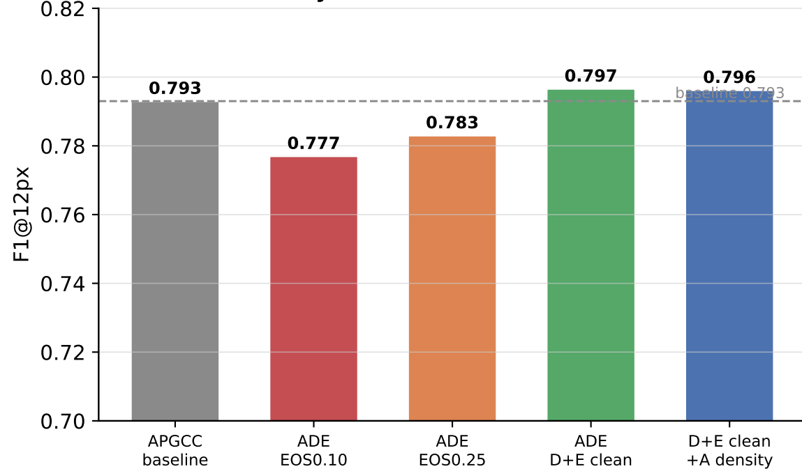
Localization: only D+E clean reaches/exceeds baseline
