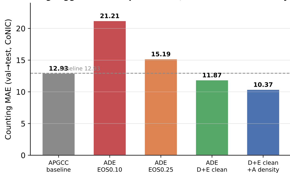
Counting: aggressive recipe harmful; D+E clean + A density best
