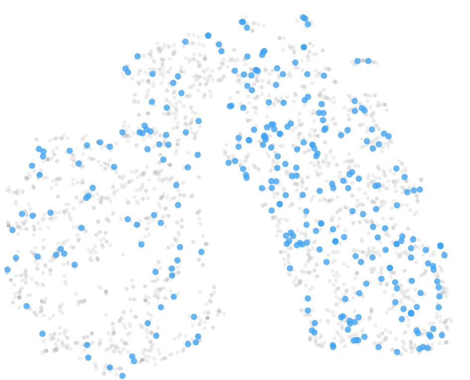
BRAIN-Coreset 10% 采样
