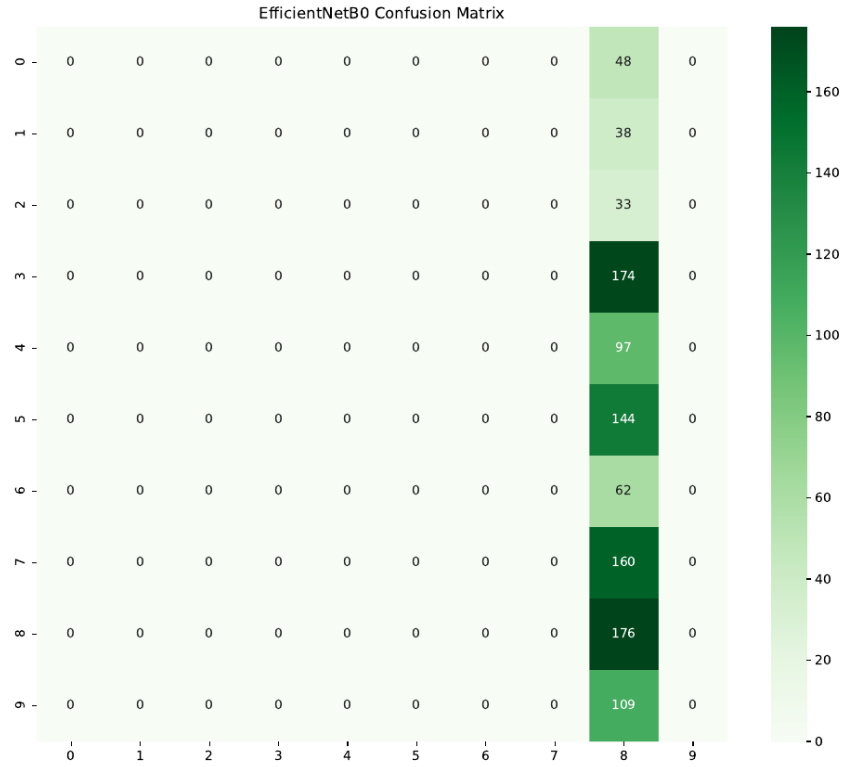
Figure 10: Confusion Matrix of the EfficientNetB0 Model, Showing Collapse to the Majority Class
