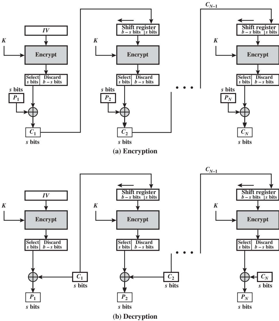
Figure 6.5 s -bit Cipher Feedback (CFB) Mode
