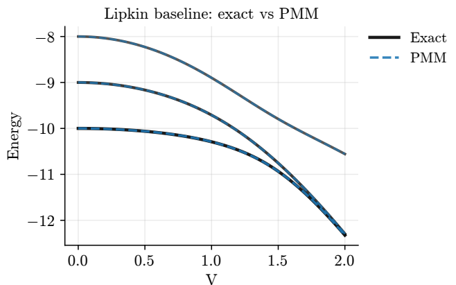
Figure 1. Baseline static Lipkin model experiment, with N = 20 , k = 3 , V \in [0, 2] and PMM dimension n = 10 .
