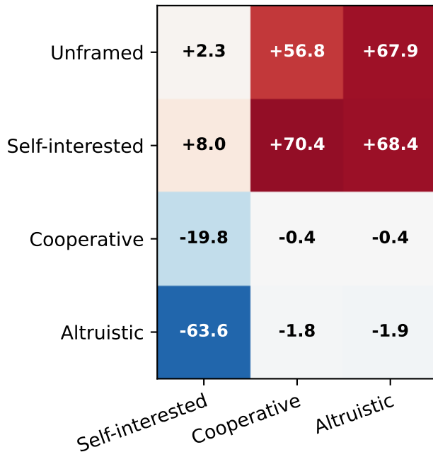
Rule-based policy
