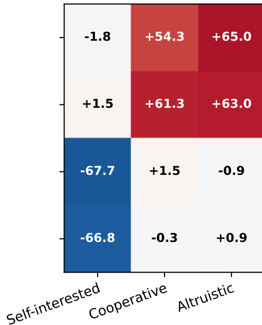
Rule-based policy
