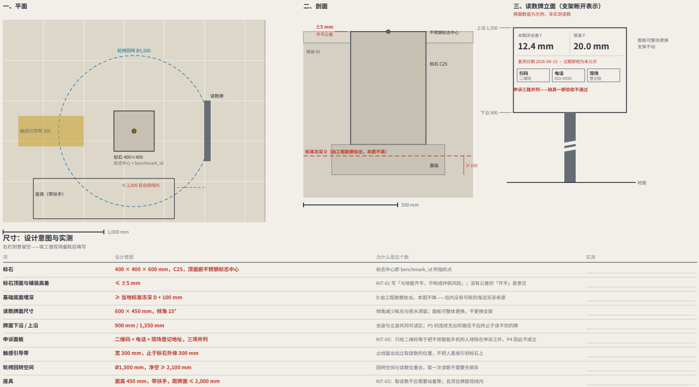
FIG.16 The benchmark and its reading plate, as a construction detail
