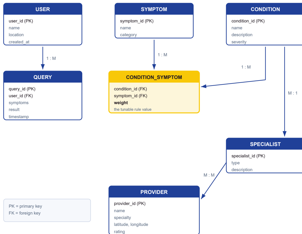
Figure 4.4: Entity relationship diagram.
