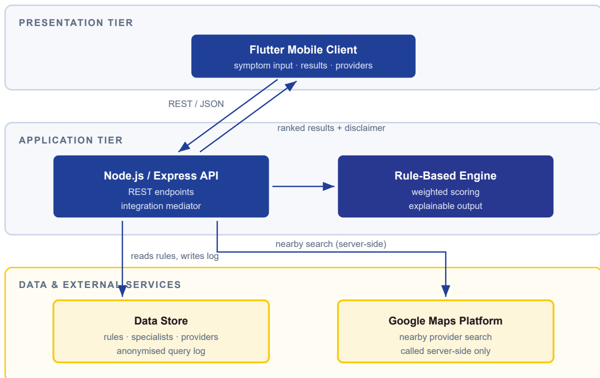
Figure 4.1: High-level architecture of the delivered system.
