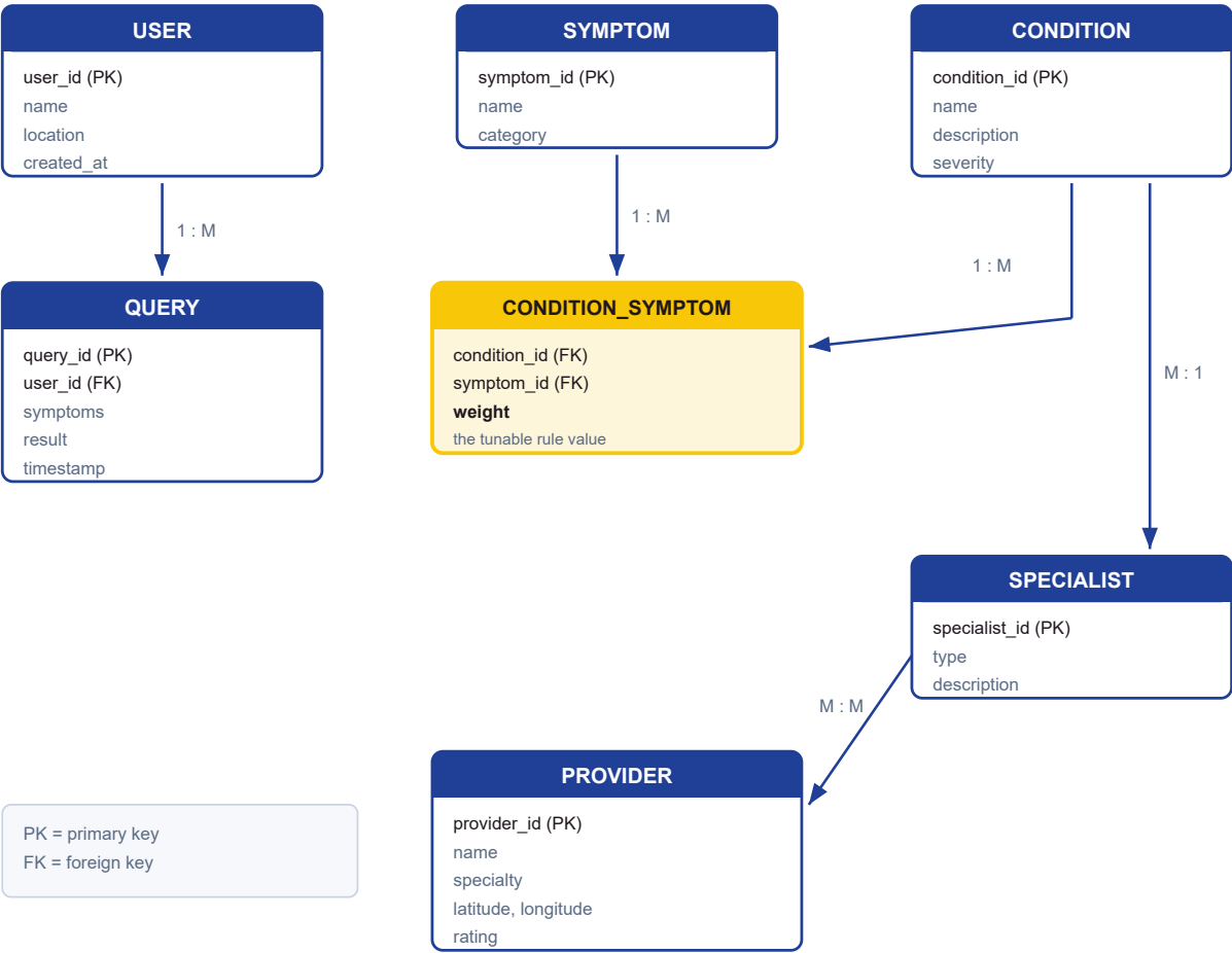
Figure A.1: Entity relationship diagram.
