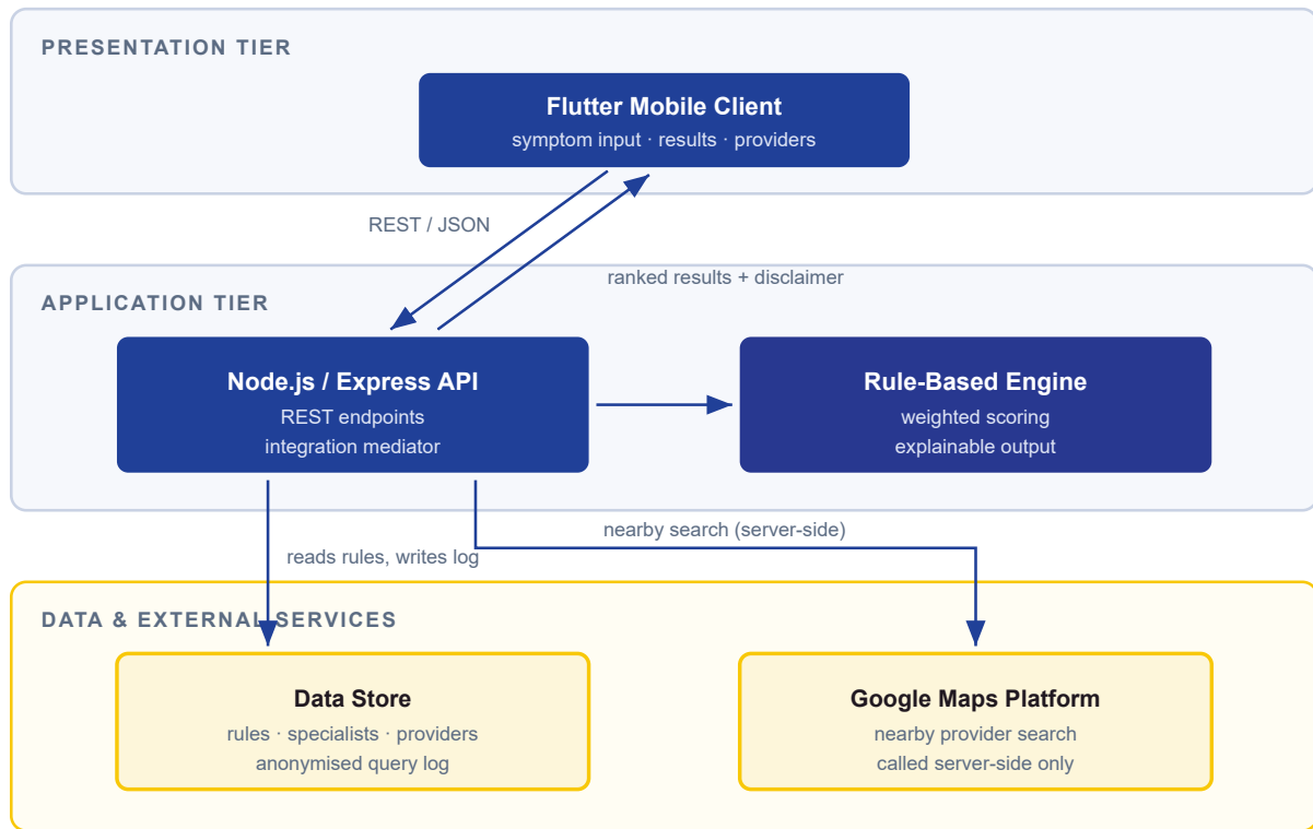
Figure 4.1: High-level architecture of the delivered system.
