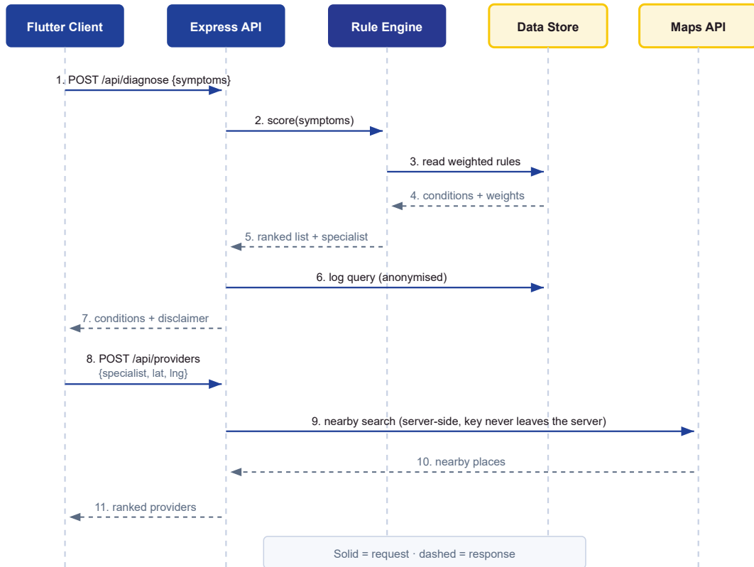
Figure 4.5: End-to-end data flow between client, API, engine and services.
