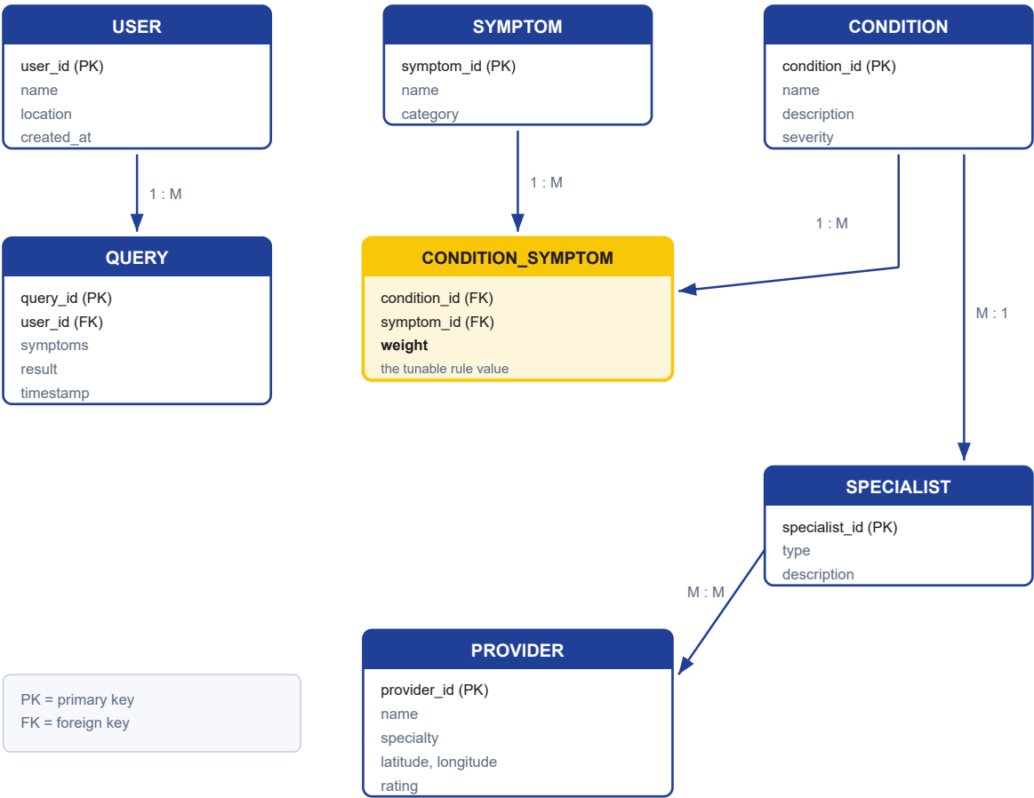
Figure A.1: Entity relationship diagram.
