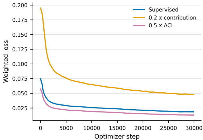
ACPD-v2 objective components
