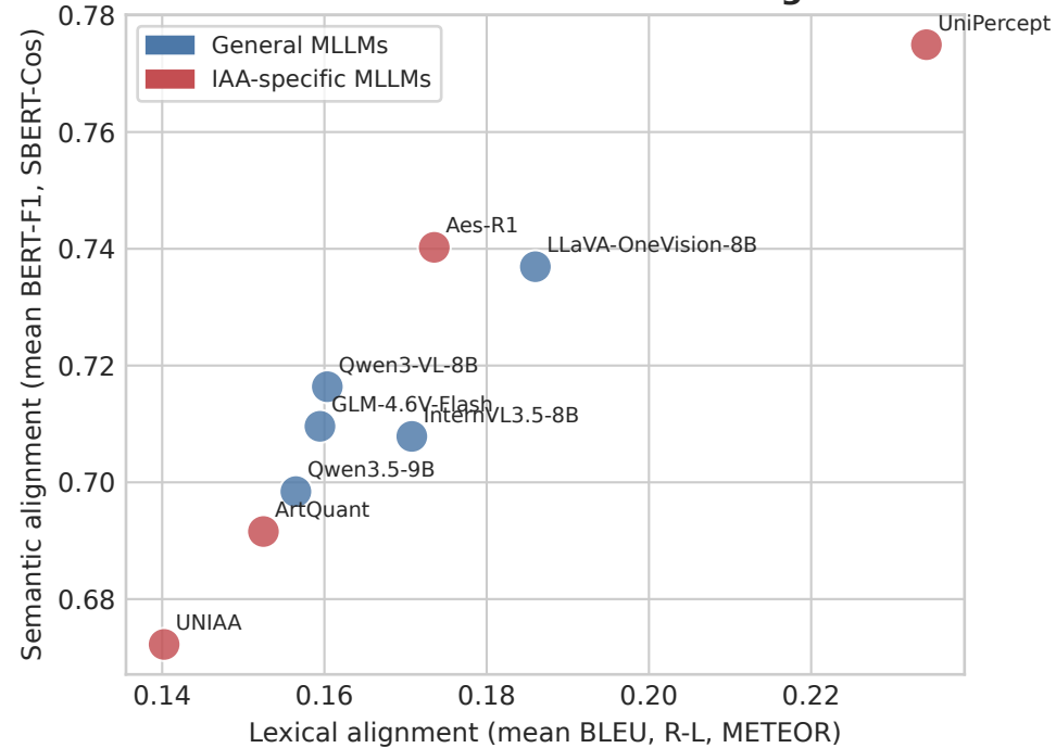
ArtiMuse: Lexical vs. Semantic Alignment
