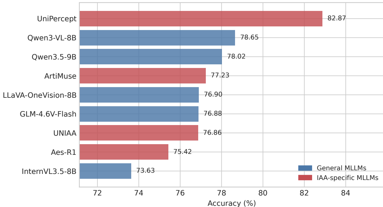
UNIAA-Bench Perception (strict-v2)
