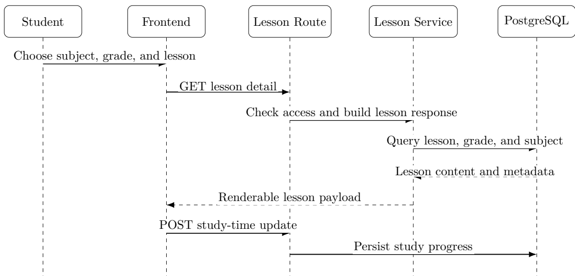
Figure 3.15: Sequence diagram for studying a lesson
