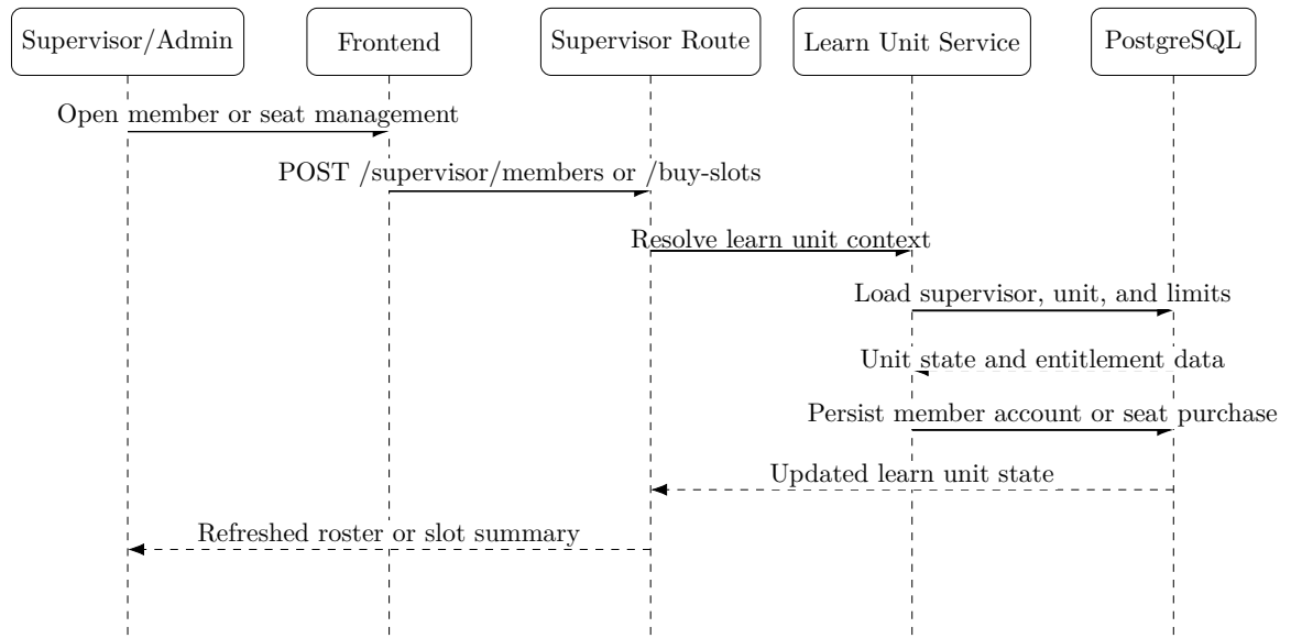
Figure 3.20: Sequence diagram for managing learning unit members and seats
