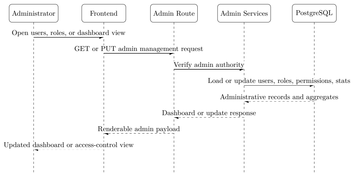
Figure 3.21: Sequence diagram for managing roles, access control, and dashboard data
