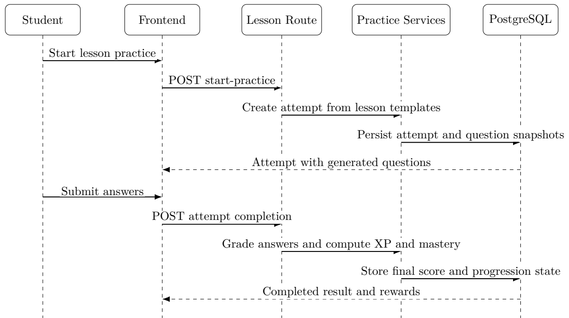
Figure 3.16: Sequence diagram for completing lesson practice
