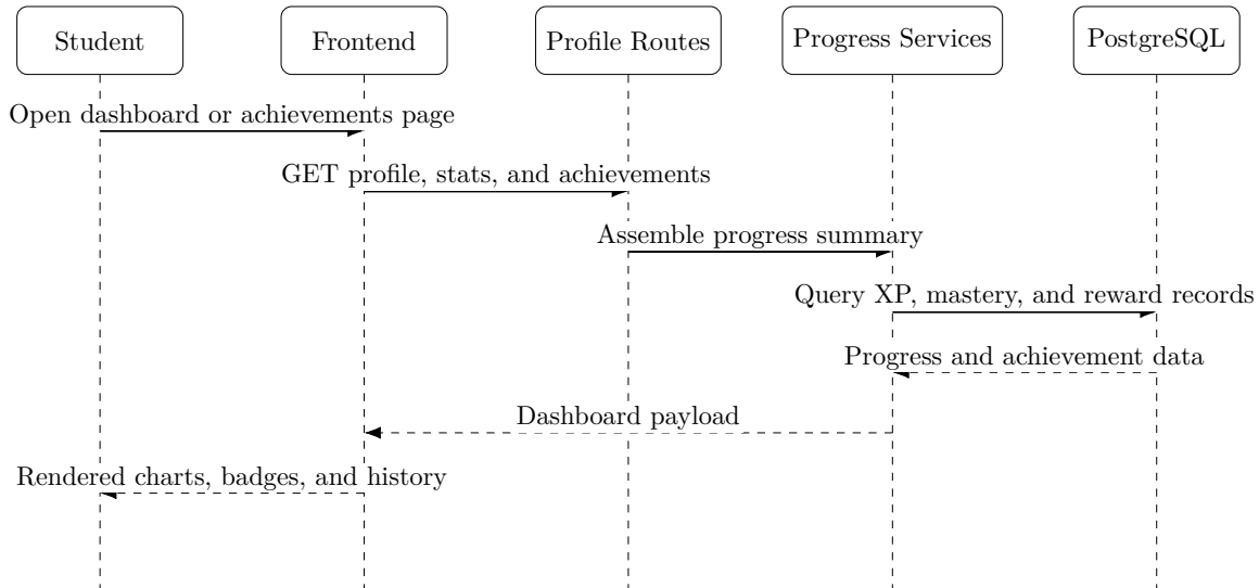
Figure 3.18: Sequence diagram for viewing progress and achievements
