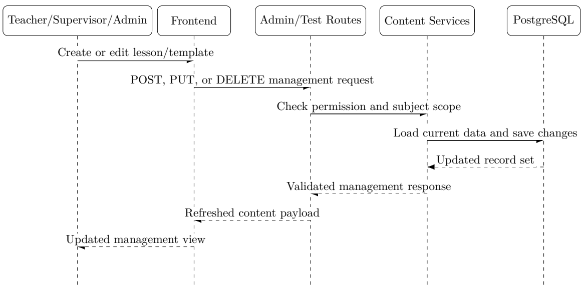
Figure 3.19: Sequence diagram for managing content and question templates
