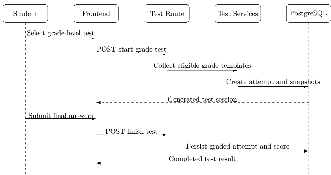
Figure 3.17: Sequence diagram for taking a grade-level test
