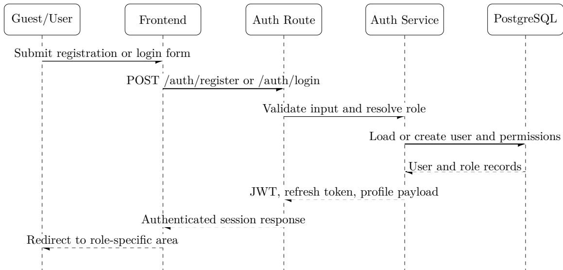
Figure 3.14: Sequence diagram for registration or login
