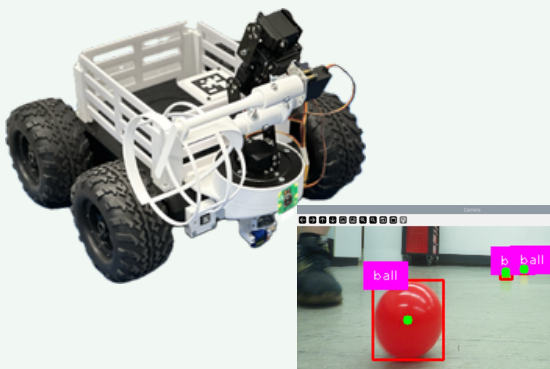
Left: Modified autonomous rover Right: Custom YOLO object-detection output
