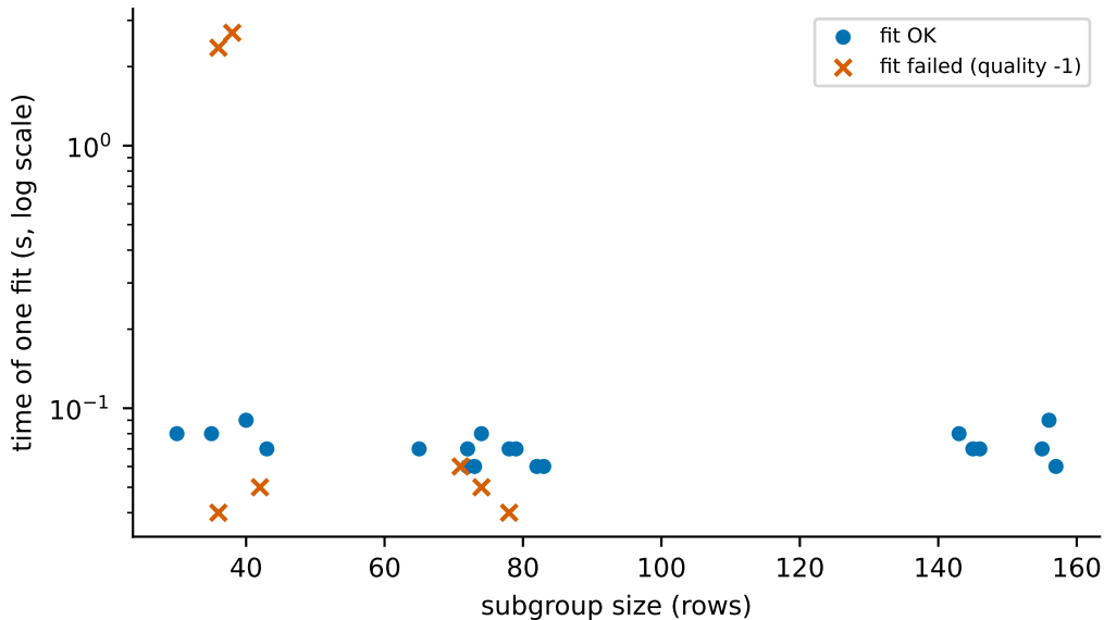
Failed fits take 80% of all fit time (HS, min. size 30)
