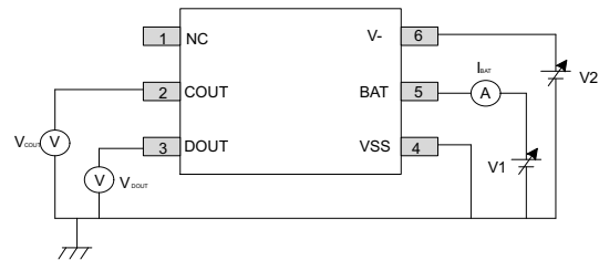
Figure 7-4. Test Circuit 2
