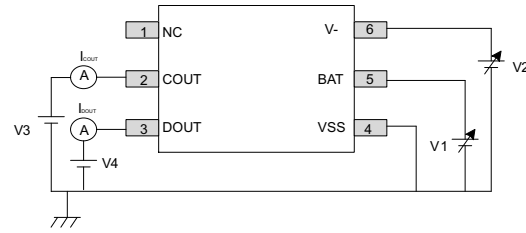
Figure 7-6. Test Circuit 4
