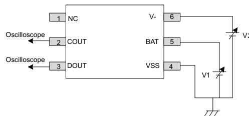
Figure 7-7. Test Circuit 5
