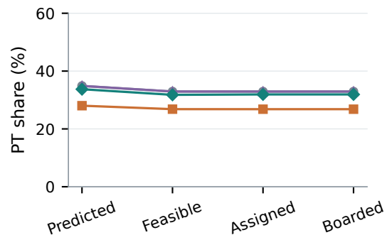
b MNL-S + neural timing
