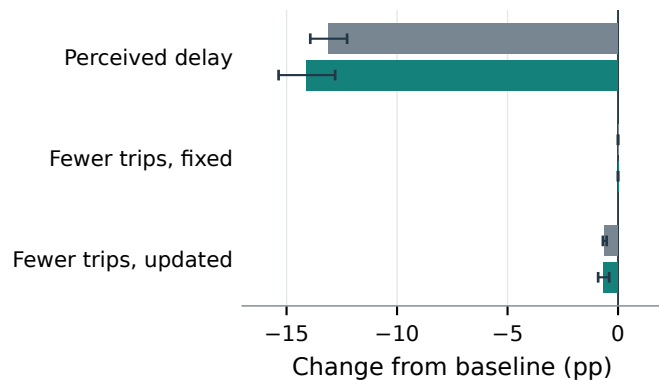
c Response to each change
