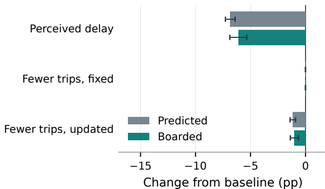
d Response to each change
