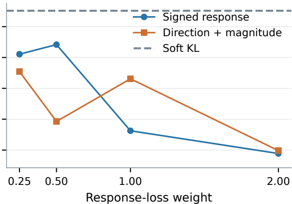
b Select by validation response
