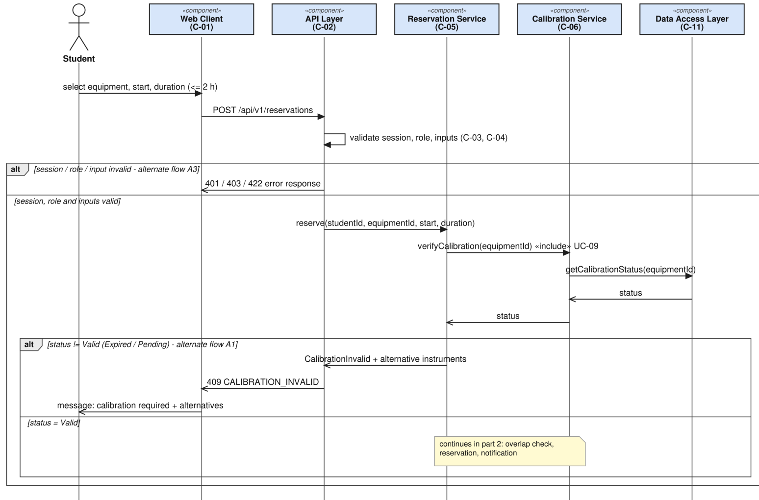
Sequence Diagram 1 (part 1 of 2) - UC-03 Reserve Equipment Slot: request validation and calibration check
