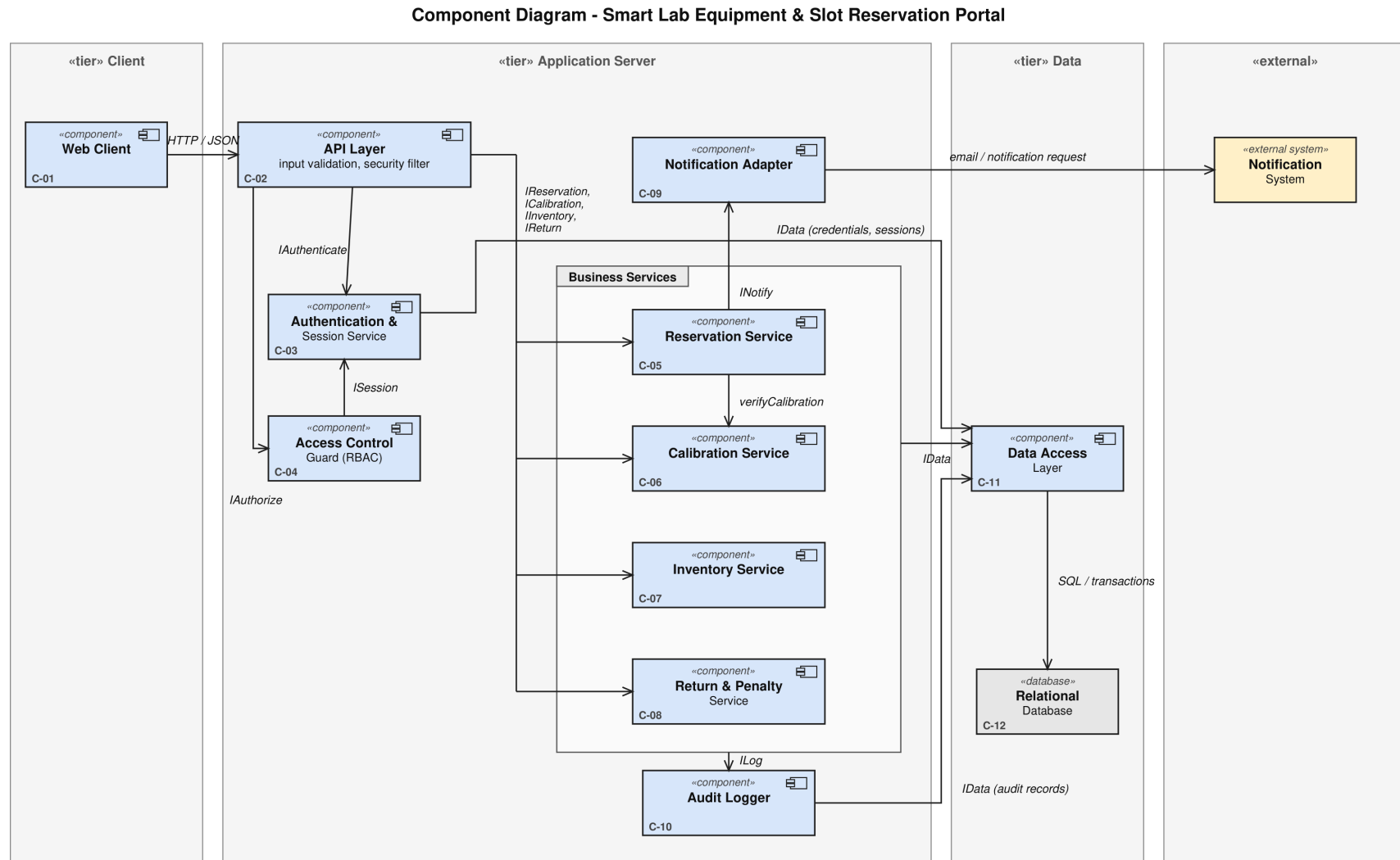
Figure 2 – UML Component Diagram (draw.io source: diagrams/component.drawio)
