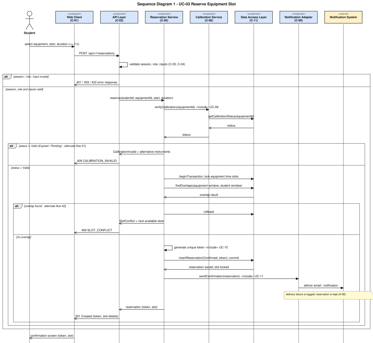
Figure 3 – Sequence Diagram 1: Reserve Equipment Slot
