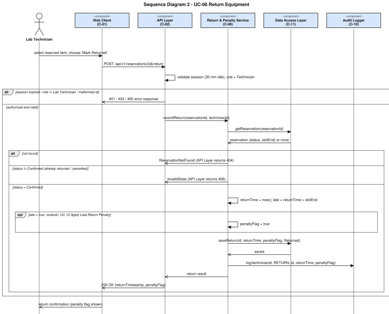
Figure 4 – Sequence Diagram 2: Return Equipment
