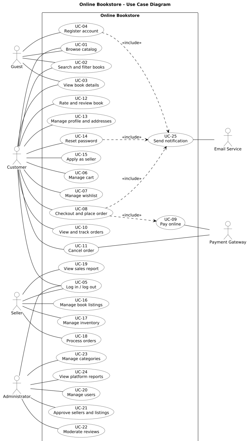
Figure 1. Use case diagram for Online Bookstore. Actors are associated explicitly with their use cases; there is no generalization between actors. Dashed arrows labelled «include» show included use cases.
