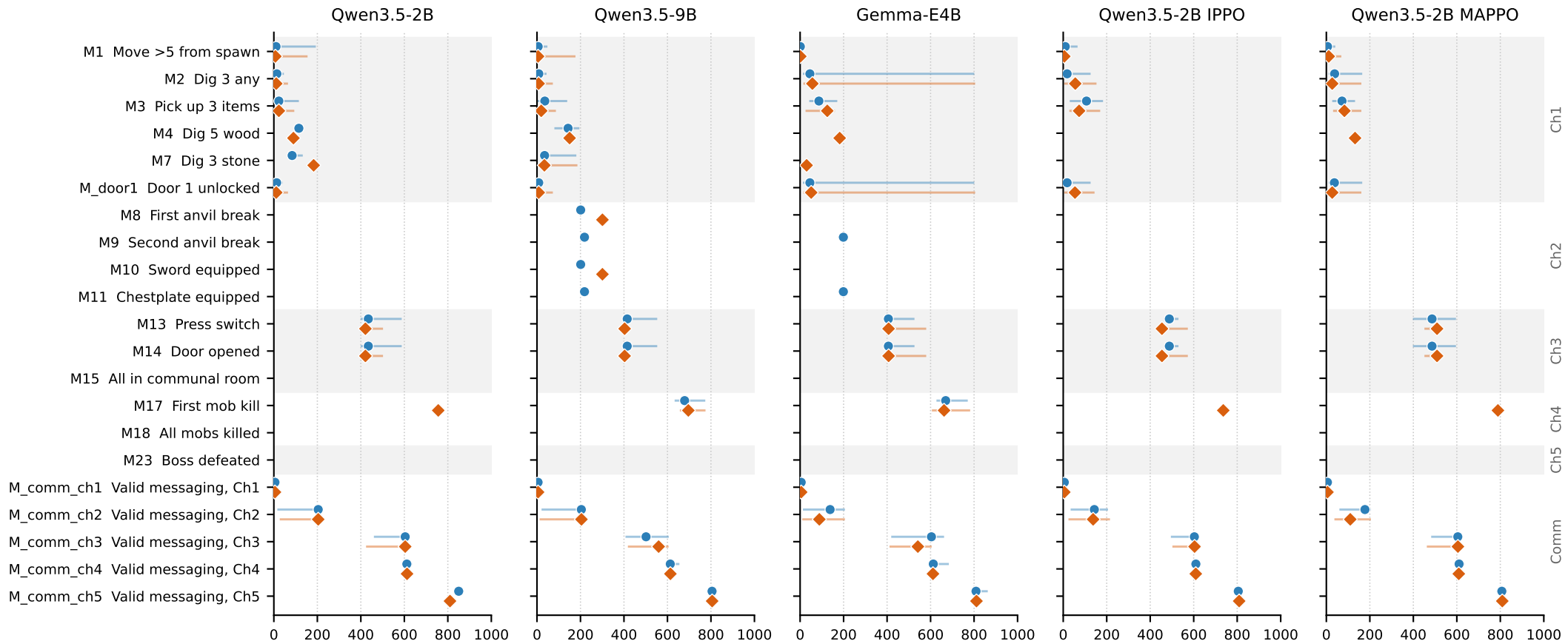
Within-episode step of first completion
