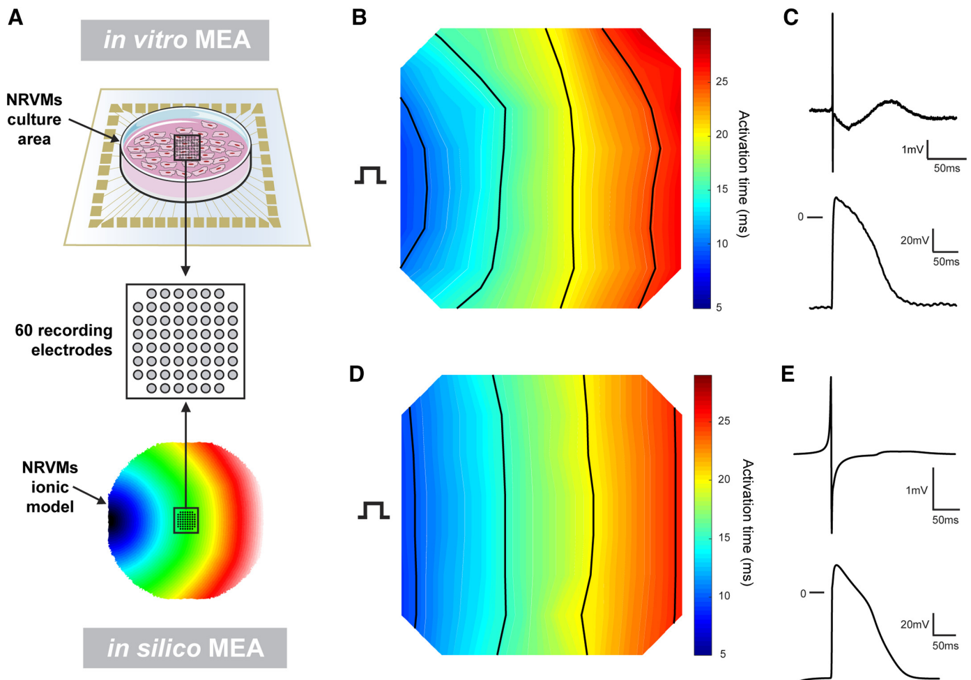
Figure 1. In silico multielectrode array (MEA) model of neonatal rat ventricular myocytes (NRVMs). A: study design: neonatal rat ventricular myocytes (NRVMs) were cultured on a multielectrode array (MEA, 60 recording electrodes) and electrical activity was measured on day 4. Simulations were performed using an NRVM ionic model with similar cell density and electrode grid characteristics. B: activation map from the 60 electrodes grid on which neonatal rat ventricular myocytes were cultured. Local activation time was defined as the time of the maximum downslope of the field potential. Activation times according to the scale on the right. C: field potential was recorded from one of the electrodes of the MEA ( C, top ) and action potential ( C, bottom ) was obtained by microelectrode recording of cultured NRVMs in the same MEA. D: activation map from the electrode grid area of the in silico model of NRVMs, field potential from one electrode ( E, top ) and transmembrane recording ( E, bottom ) from the electrode location. Isochrones at 5 ms. Activation times according to the scale on the right.
