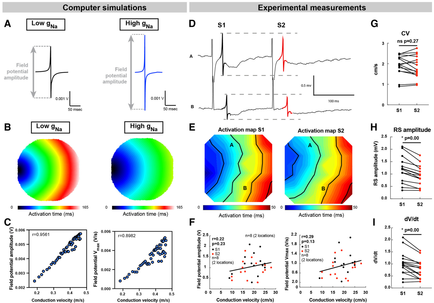
Figure 2. Field potential amplitude correlates with conduction velocity. A: field potentials obtained from simulations in which the fast sodium channel conductance ( g_{Na} ) was modified by a factor of 1.05 (left, low g_{Na} ) and 5.15 (right, high g_{Na} ) of baseline conditions. B: example of two activation maps constructed from simulations in which the fast sodium channel conductance ( g_{Na} ) was modified by a factor 1.05 (left, low g_{Na} ) and 5.15 (right, high g_{Na} ) of baseline conditions. Activation times according to the scale below. C: correlation between field potential amplitude (left), field potential maximum down-slope velocity ( V_{max} ; right), and conduction velocity. Nonparametric Spearman's correlation. r = 0.9561 , P < 0.0001 , n = 49 for field potential amplitude. D: electrograms recorded from a neonatal rat cardiomyocyte monolayer from locations A and B as indicated in the activation maps of E . F: correlation between field potential amplitude (left), field potential maximum down-slope velocity ( V_{max} ) (right), and conduction velocity. Nonparametric Spearman's correlation. r = 0.22 , P < 0.23 for field potential amplitude. The bar graphs show local conduction velocity ( G ), RS amplitude ( H ), and dV/dt_{min} of down-slope of RS complex ( I ) at locations A and B before and after premature stimulations (black vs. red dots). A paired t test was used to determine significance.
