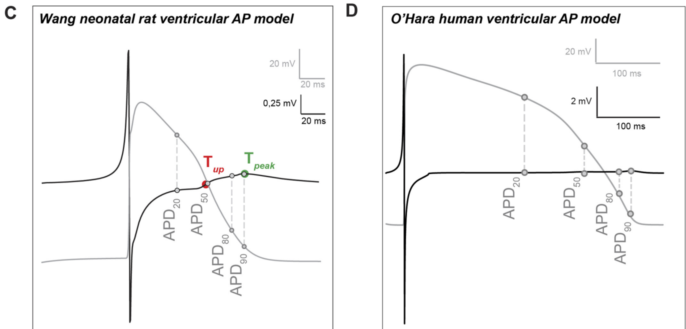
Figure 3. Comparison of field potential and action potential characteristics. A: scatterplot between T up and APD 50 , and T peak and APD 90 determined in field potentials and transmembrane potentials recorded using glass-pipette microelectrodes. Recordings were done in 15 monolayers at a spontaneous frequency varying between 450 and 1,000 ms intervals. Example of field potential and action potential of NRVMs obtained in vitro ( B ) and in silico using the Wang and Sobie model ( C ), and the O'Hara model ( D ). Action potential duration at 20, 50, 80, and 90% of repolarization (APD 20 , APD 50 , APD 80 , and APD 90 ) are indicated on both panels. T up indicates the time between activation (maximum downslope of the field potential) and maximal upstroke of the T wave. T peak indicates the time between activation and peak of the T wave.
