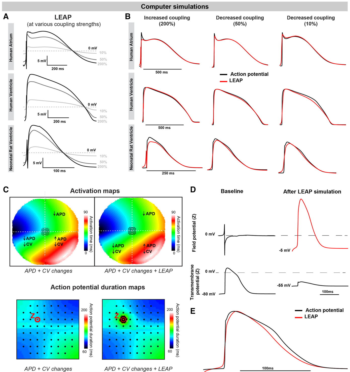
Figure 6. Local extracellular action potential (LEAP) in the presence of electrophysiological heterogeneities. A: LEAP simulations using a human atrial and ventricular, and neonatal rat ventricular model. Simulations were performed at 10%, 50%, and 200% of baseline intercellular coupling. B: overlay of transmembrane potential (black) and LEAP (red) at the aforementioned coupling strengths using the aforementioned action potential models. C: activation and action potential duration maps (zoomed in on electrode grid) obtained action potential duration (APD) and conduction velocity heterogeneity were induced in the monolayer by modifying currents in the southeast (SE), southwest (SW), and northeast (NE) quadrants, before and after LEAP simulation. Specifically, conduction velocity was reduced in the SE and SW quadrants; APD was prolonged in the SE quadrant and shortened in the NE and SW quadrants. Shortening or prolongation of the APD was obtained by increasing or decreasing the conductance of the inward-rectifier potassium channels ( I_{K1} ) by a factor of 5 compared with the baseline. Conduction slowing was obtained by decreasing the fast sodium channel conductance ( g_{Na} ) by a factor of 3 compared with baseline. D: field potentials before (left) and after LEAP simulation (right) extracted from point Z. Transmembrane potentials before (left) and after LEAP simulation (right). E: overlay of the transmembrane potential before LEAP simulation and the field potential after LEAP simulation. APD, action potential duration.
