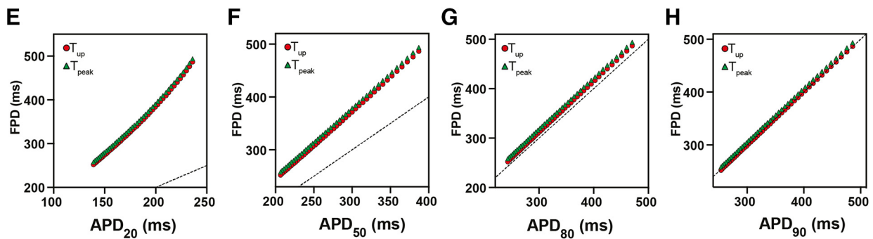
Figure 4. Field potential duration correlates with action potential duration (APD) 20, 50, 80, and 90% of repolarization. Correlation between APD 20 (A), APD 50 (B), APD 80 (C), APD 90 (D), and field potential duration (at T_{\text{peak}} or T_{\text{up}} ) in the in silico Wang neonatal rat ventricular model (A–D) and in the O'Hara human ventricular model (E–H). To prolong the APD, the (slow and rapid) delayed rectifier potassium channel conductances were modified by a factor of 1.1 to 4.8 and 0.5 to 1.4 of baseline conditions in the rat and human models, respectively. T_{\text{up}} indicates the time between activation (maximum down-slope of the field potential) and maximal upstroke of the T wave. T_{\text{peak}} indicates the time between activation and peak of the T wave. The dotted line indicates the line of identity. In neonatal rat ventricular myocytes (NRVMs), the APD 90 correlates with T_{\text{peak}} , and APD 50 correlates with T_{\text{up}} . E–H: example of field potential and action potential obtained from the in silico O'Hara ventricular model; APD 20 (E), APD 50 (F), APD 80 (G), and APD 90 (H) are indicated.
