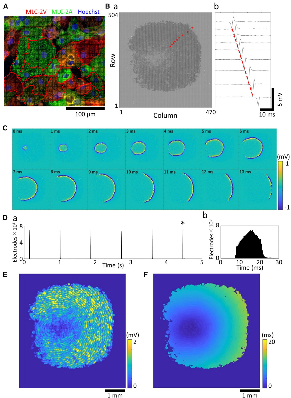
Fig. 1. Field potential imaging in human iPSC-derived cardiomyocytes. A) Immunostaining images. Red: Myosin Light Chain 2 Ventricular (MLC-2V); Green: Myosin Light Chain 2 Atrial (MLC-2A); Blue: Hoechst 33258. B) a) Extracellular potential waveforms recorded from 236,880 electrodes. b) Extracellular potential waveform from the electrode marked with a star. C) Time-lapse of the potential heatmap for each sampling point across all electrodes during a single beat. D) a) Histogram of the number of active electrodes over 5 s (bin size = 0.5 ms). b) Enlarged view of a single beat marked with an asterisk in a). E) Heatmap of the maximum voltage amplitude during a single beat. F) Delay map of voltage peak timing during a single beat.
