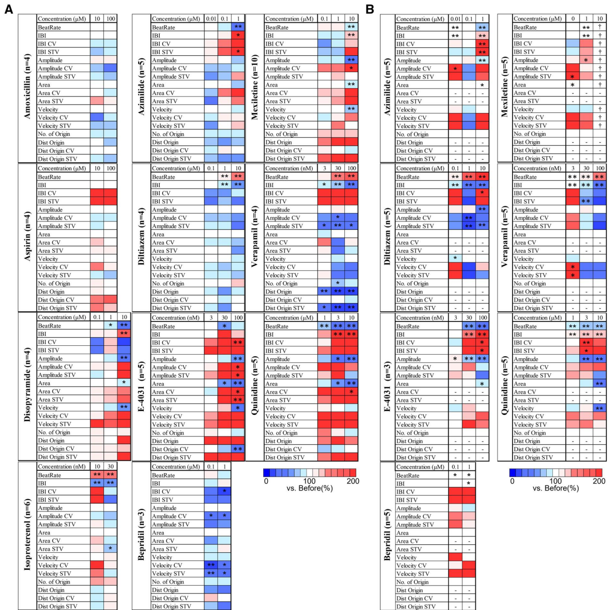
Fig. 5. Heatmaps of beating parameter changes in the acute response to cardiotoxic and non-cardiotoxic compounds in human iPSC-derived cardiomyocytes. A) UHD-CMOS-MEA recordings for 11 compounds, showing changes in 17 beating-related parameters across multiple concentrations. B) Conventional MEA results for the corresponding compounds. Each value is normalized to 100% based on pre-treatment values for each parameter. One-way ANOVA followed by Dunnett's post hoc test was performed. * P < 0.05 vs. before, ** P < 0.01 vs. before. "—" indicates parameters not calculable due to insufficient spatial resolution in the conventional MEA system. "+" indicates values not available due to complete cessation of spontaneous beating after compound administration.
