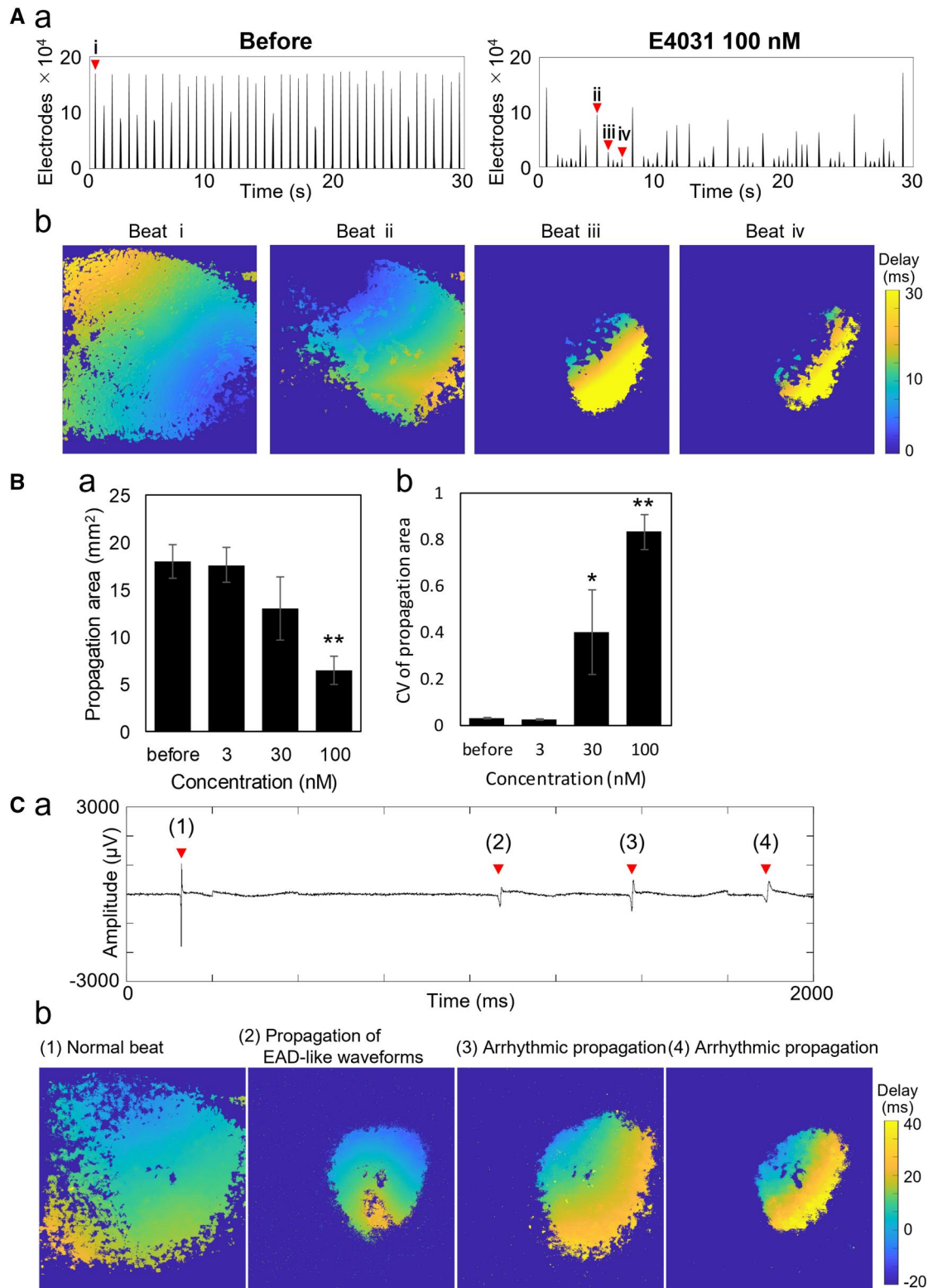
Fig. 4. Decrease in propagation area and detection of EAD-like waveforms induced by E-4031. A) a) Histogram of the number of active electrodes over 30 s before (left) and after the treatment of 100 nM E-4031 (right). A) b) Heatmap of peak timing for each beat indicated by arrows in a). B) a) Concentration-dependent decrease in the average propagation area. B) b) Concentration-dependent increase in the coefficient of variation of propagation area ( n = 6 wells). * P < 0.05 vs. before, ** P < 0.01 vs. before. C) a) Field potential waveforms recorded after the treatment of 100 nM E-4031. C) b) Heatmap of peak timing for each beat indicated by arrows in a). 1) Beats spreading across the entire recording area. 2) Locally confined beats with EAD-like waveforms. 3) Locally confined arrhythmic propagation. 4) Locally confined arrhythmic propagation with prolonged propagation time.
