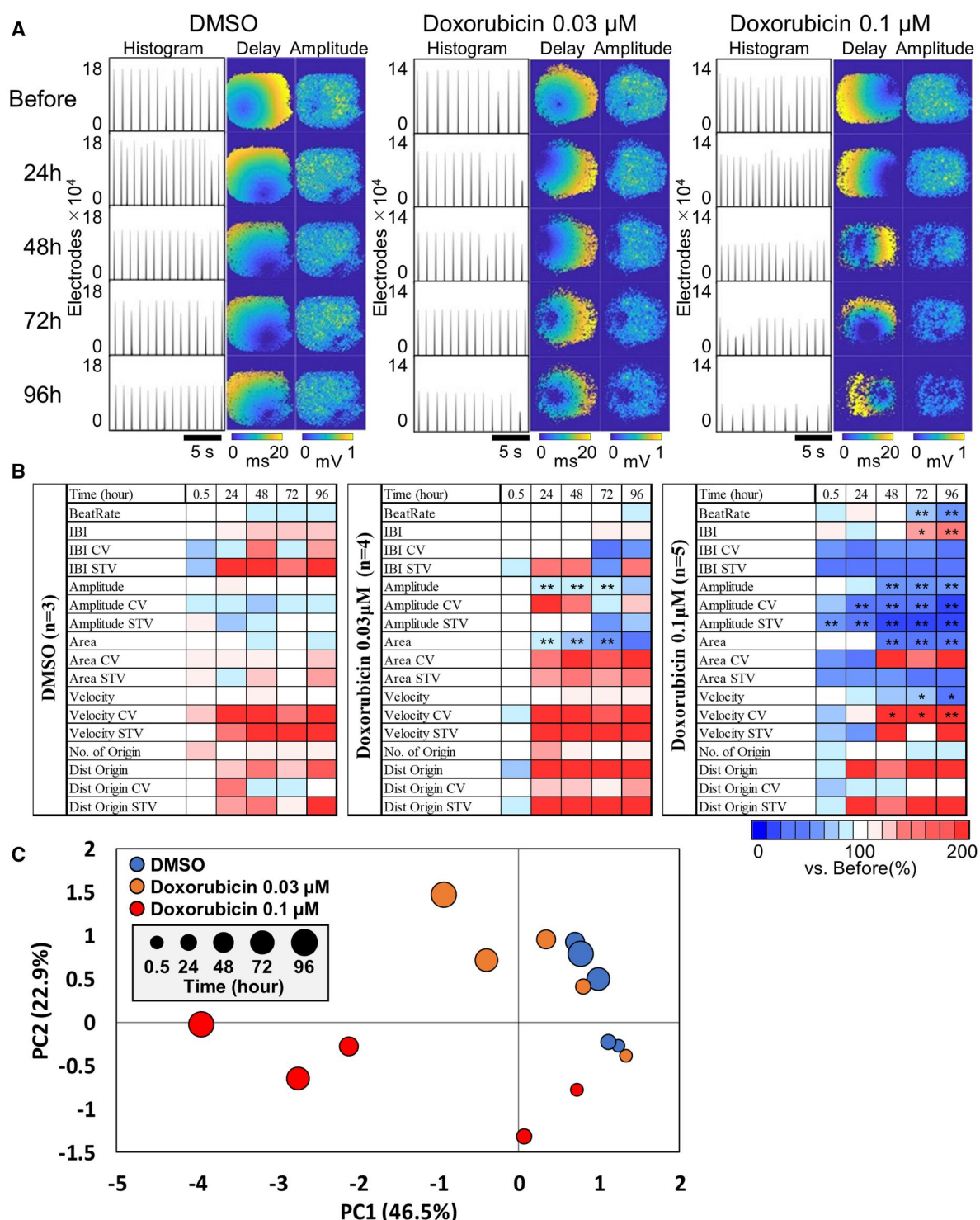
Fig. 7. Detection of chronic cardiotoxicity induced by doxorubicin. A) a) Histogram of the number of active electrodes before and after chronic treatment (left), heatmap of peak timing for a single beat (middle), and heatmap of peak amplitude for a single beat (right). B) Time-dependent heatmap of beat parameters after chronic treatment. One-way ANOVA followed by Dunnett's post hoc test was performed. * P < 0.05 vs. before, ** P < 0.01 vs. before. C) PCA plot after chronic treatment.
