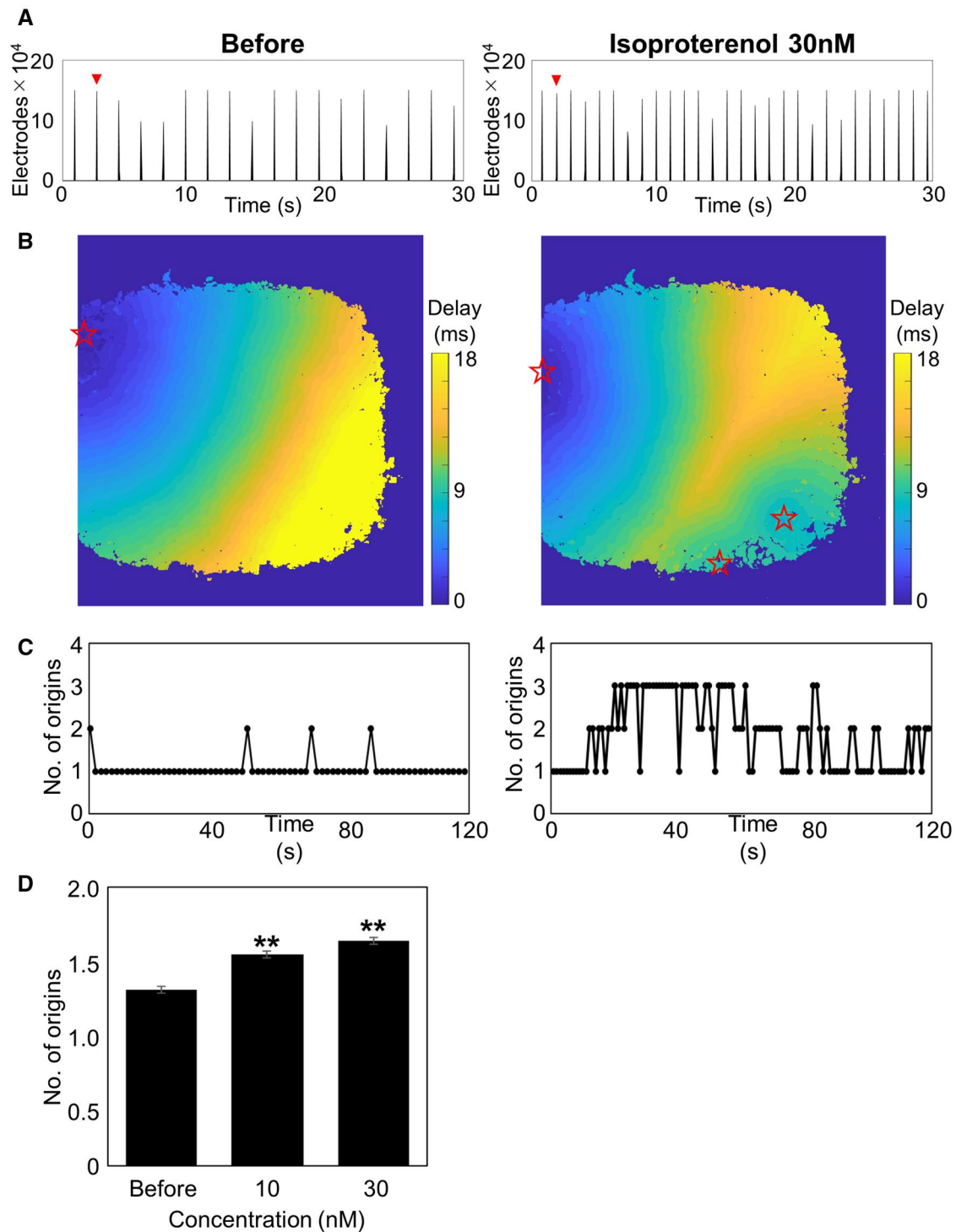
Fig. 2. Increase in the number of excitation origins induced by isoproterenol. A) Histogram of the number of active electrodes over 30 s before (left) and after the treatment of 30 nM Isoproterenol (right). B) Delay map of voltage peak timing for a single beat, where stars indicate excitation origins. C) Plot of the number of excitation origins detected over a 2-min period. D) Concentration-dependent increase in the average number of excitation origins ( n = 6 wells, ^{**}P < 0.01 vs. before).
