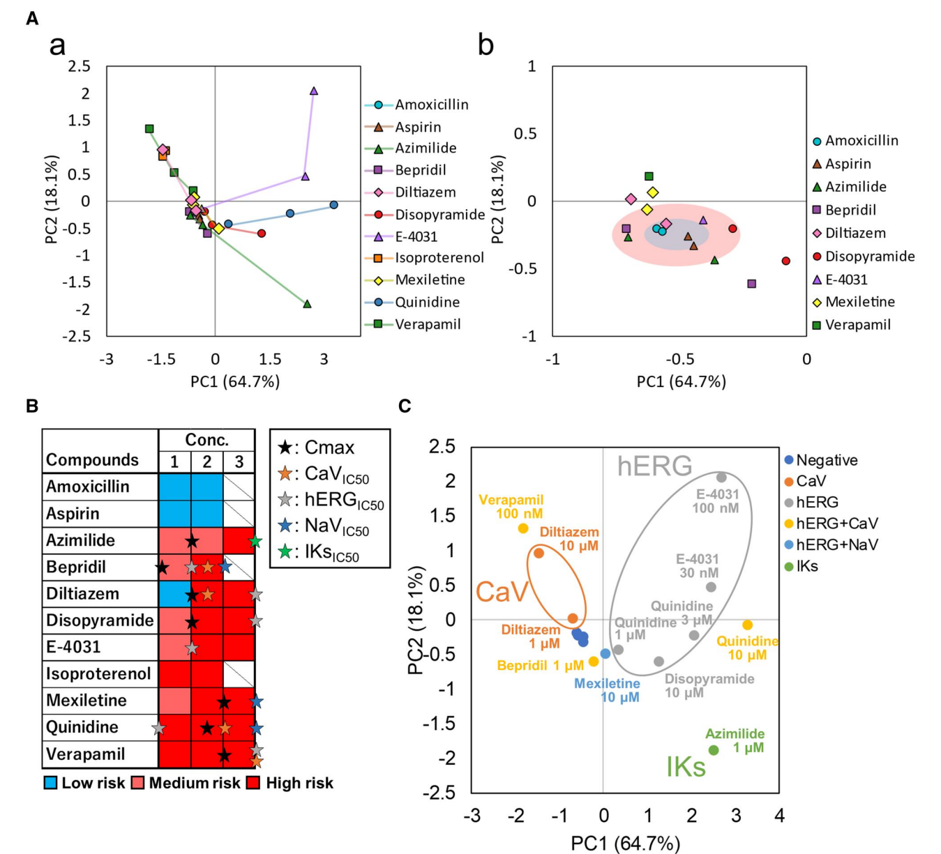
Fig. 6. Detection of cardiotoxicity and classification of mechanisms of action using PCA analysis of beat parameters. A) a) PCA plot of compounds. b) Enlarged view of the region near negative control compounds. B) Toxicity classification based on the standard deviation range of negative control compounds. Stars indicate the IC 50 and Cmax of each ion channel. C) Classification of mechanisms of action on the PCA plot based on IC 50 values.
