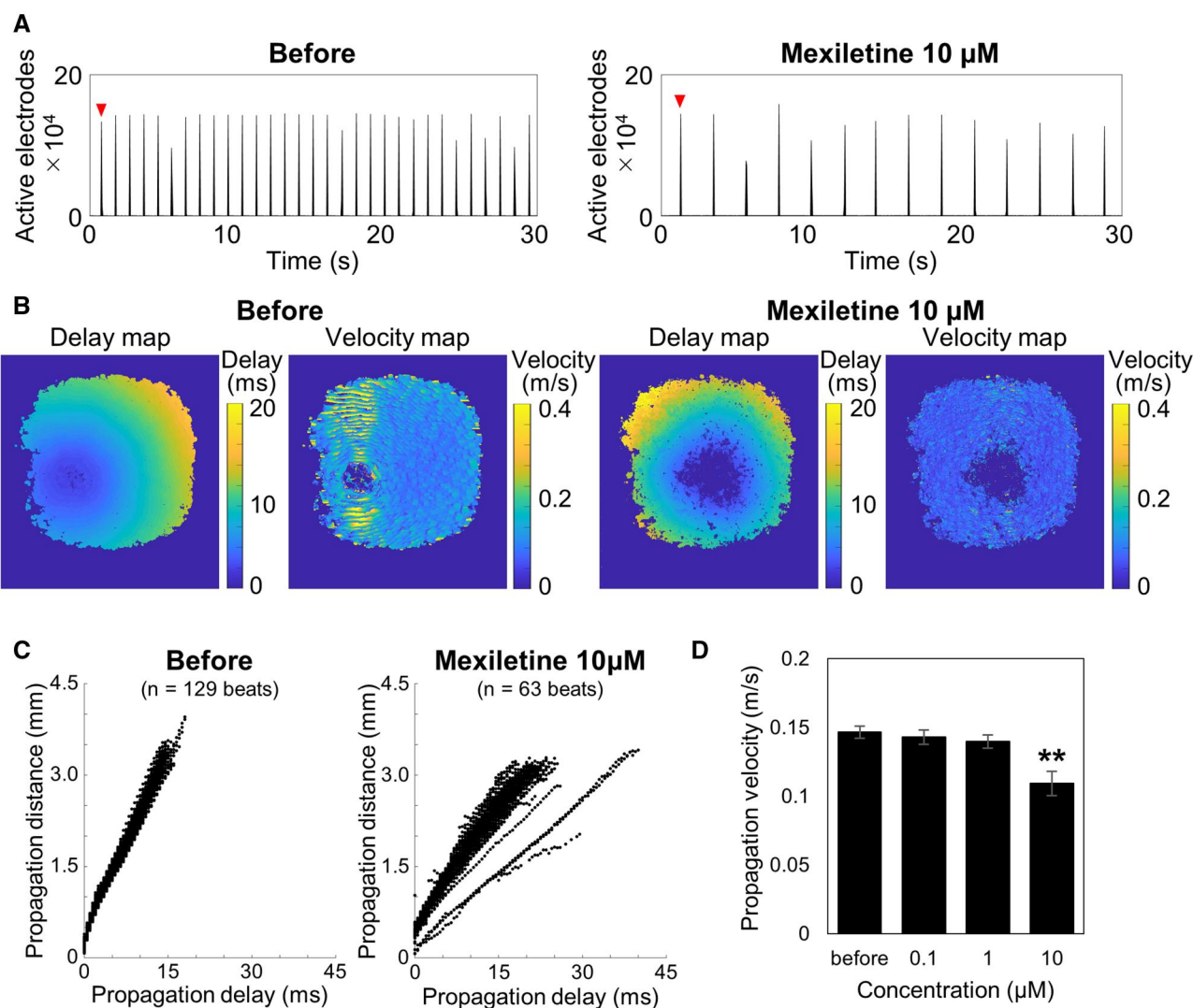
Fig. 3. Decrease in propagation velocity induced by mexiletine. A) Histogram of the number of active electrodes over 30 s before (left) and after the treatment of 10 \mu\text{M} Mexiletine (right). B) Delay map of voltage peak timing and propagation velocity heatmap for a single beat. C) Plot of propagation time and propagation distance detected over a 2-min period. D) Concentration-dependent decrease in the average propagation velocity (n = 6 wells, **P < 0.01 vs. before).
