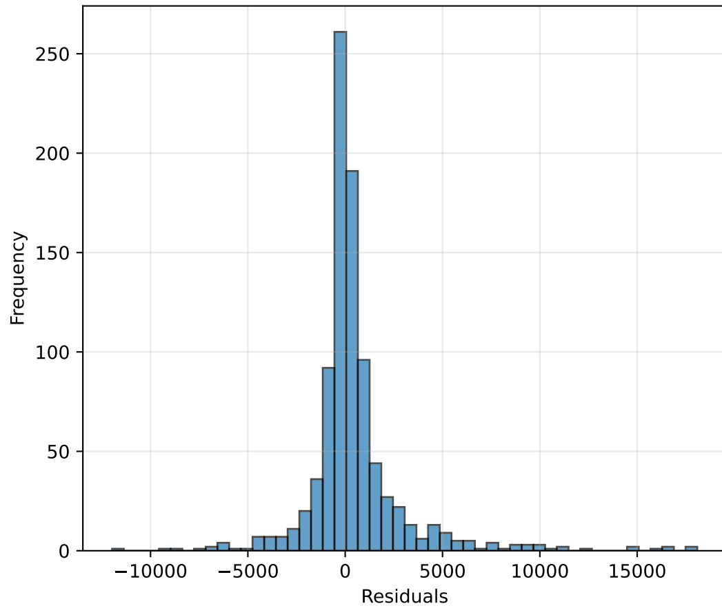
Residuals Distribution
