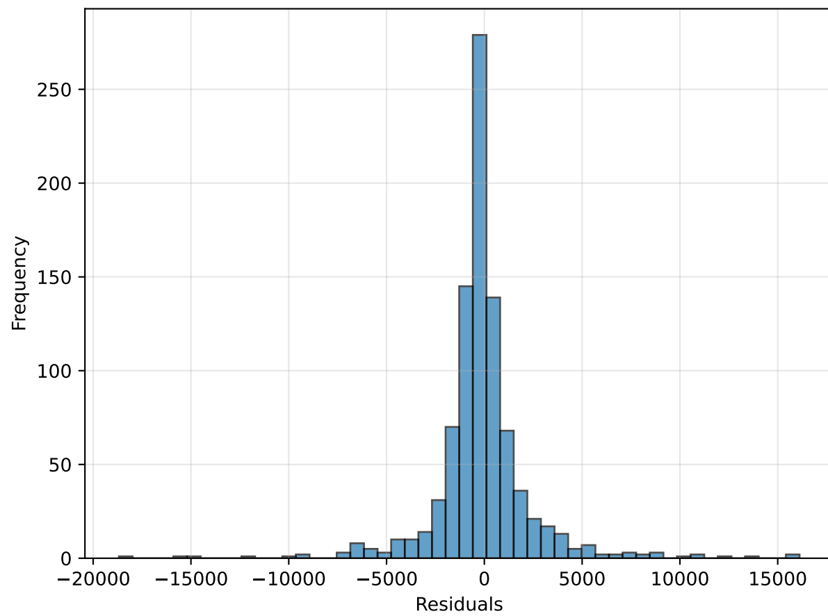
Residuals Distribution
