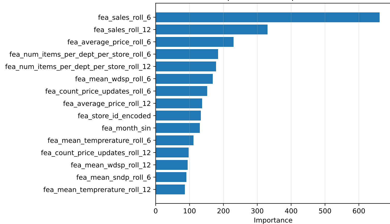
Top 15 Feature Importance
