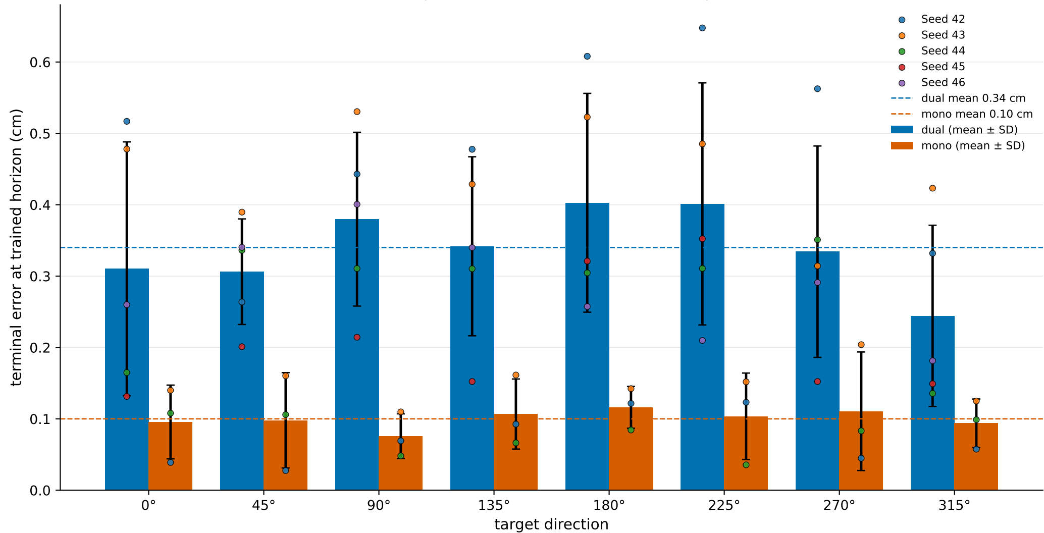
Per-direction reach accuracy (terminal error at the end of 1s episode) — dual vs mono
