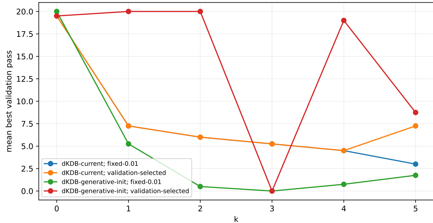
CensusIncome: best pass vs k
