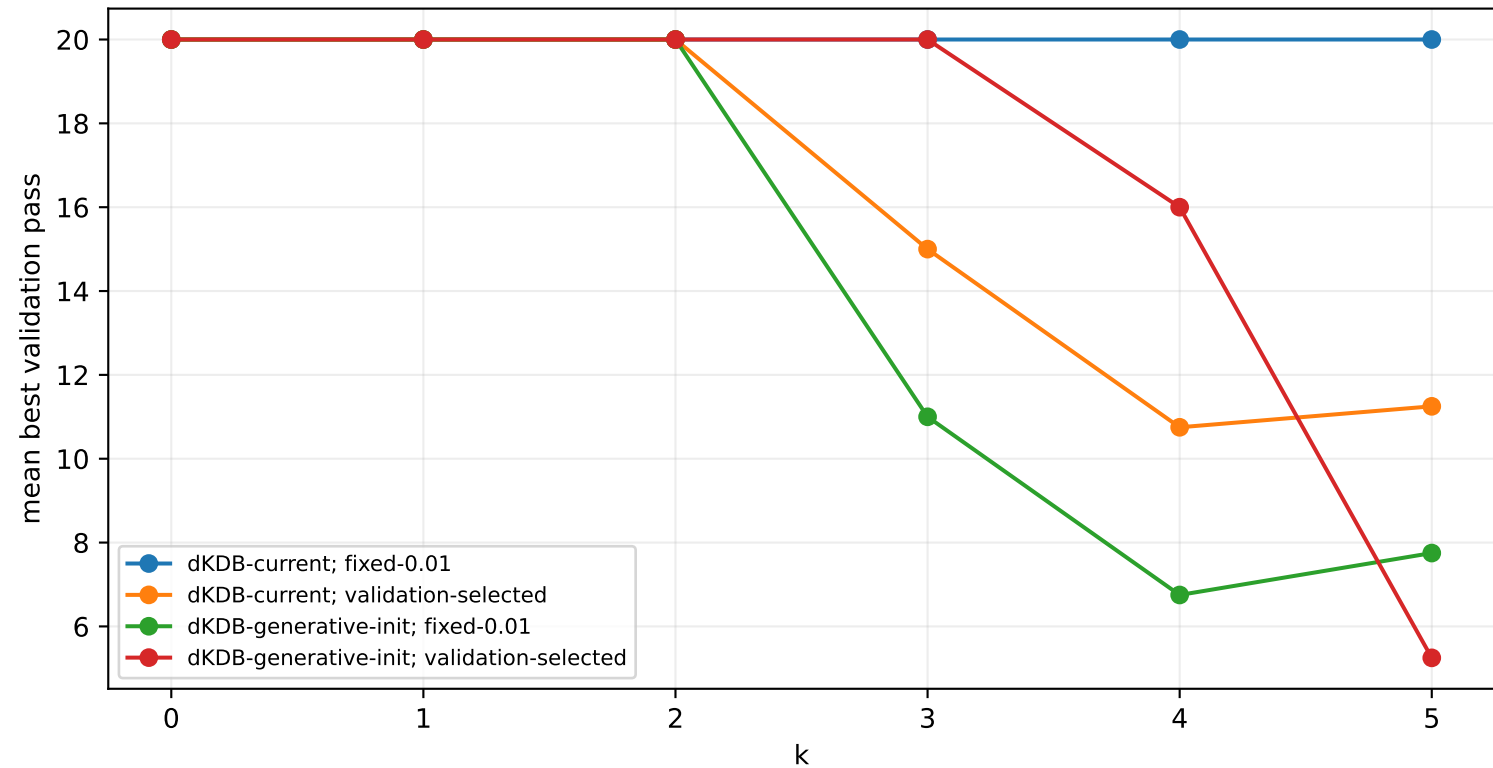
Covertypes: best pass vs k
