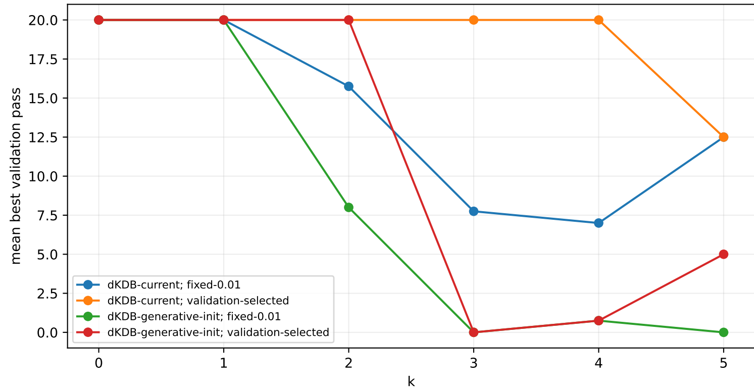
MiniBooNE: best pass vs k
