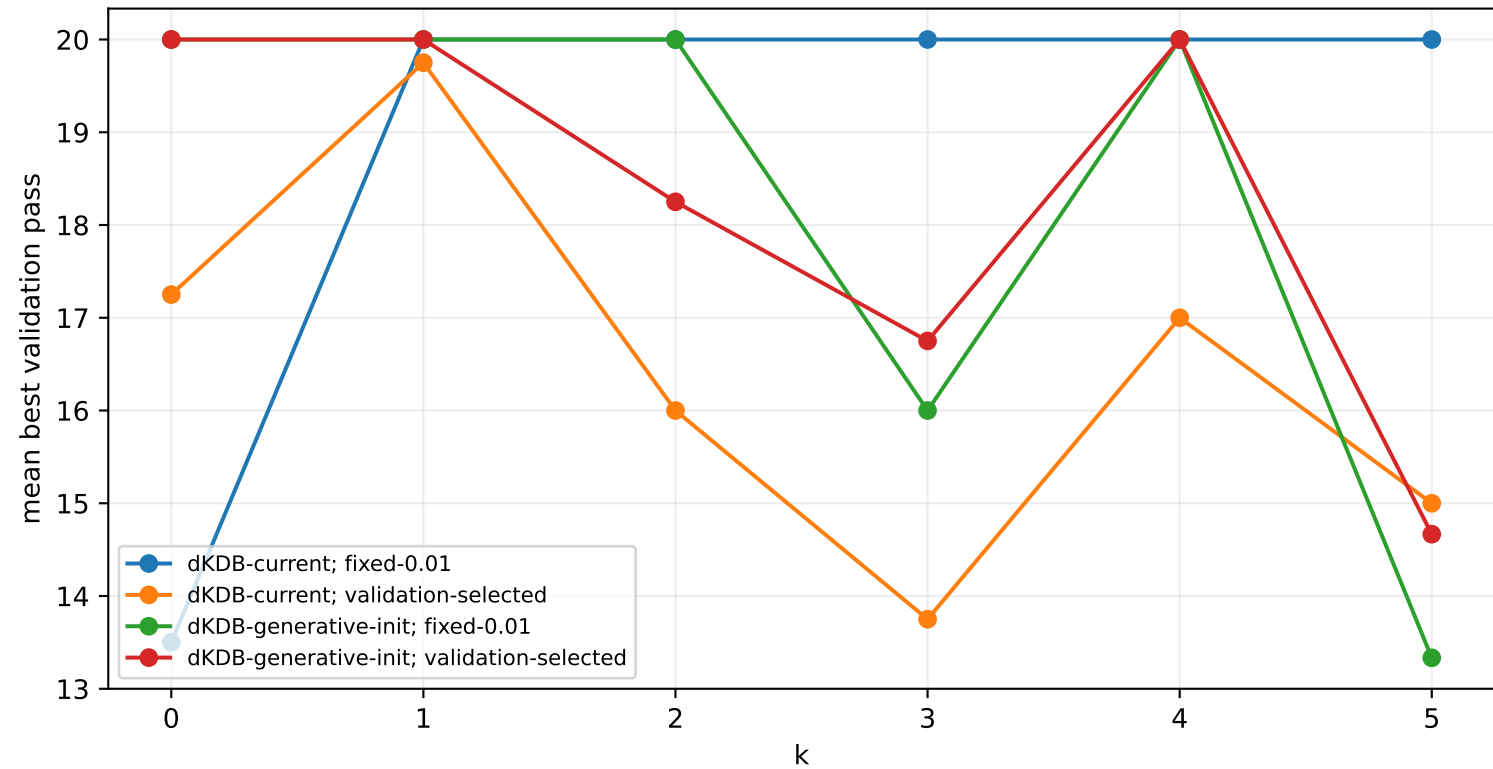
PokerHand: best pass vs k
