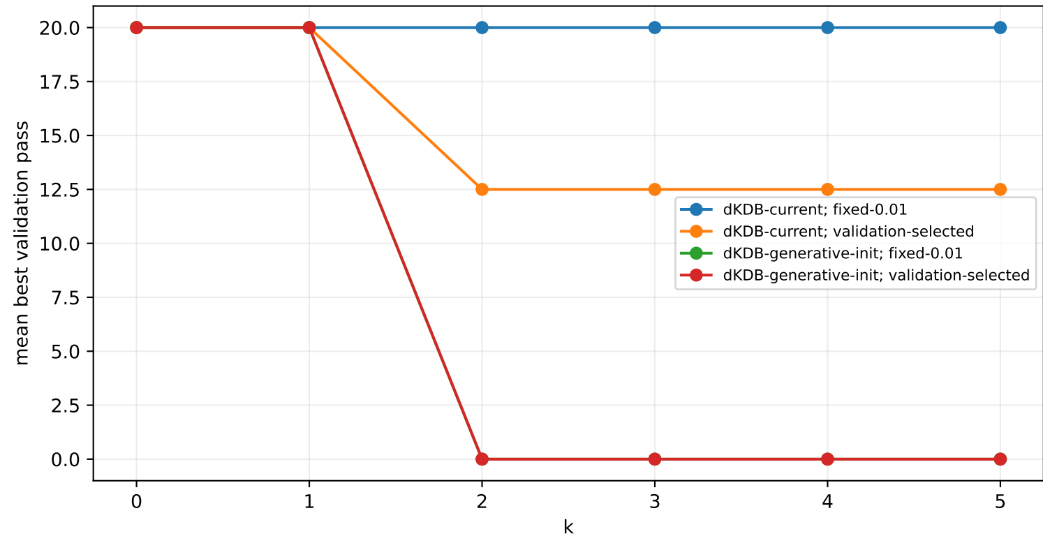
Skin Segmentation: best pass vs k
