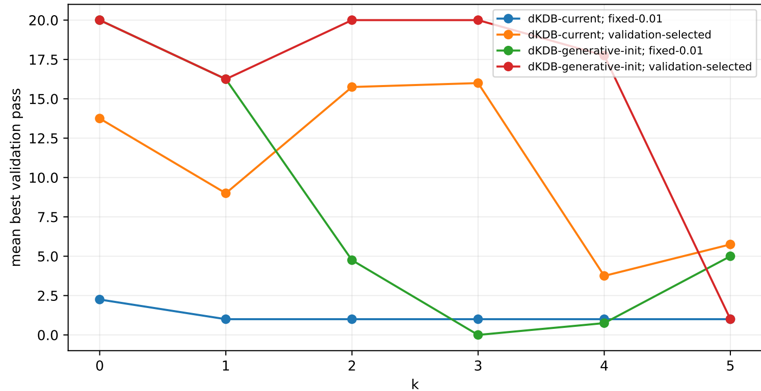
TwitterAbsoluteSigma: best pass vs k
