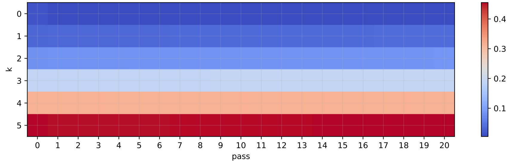
CensusIncome: Validation NLL - train NLL
